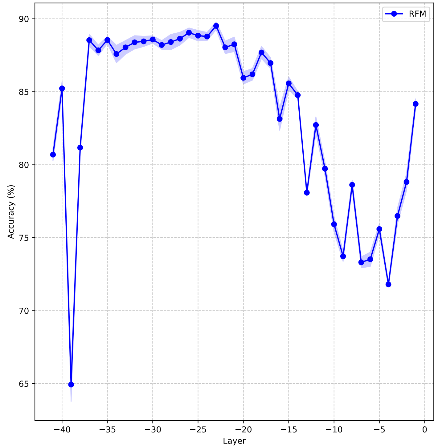
HE (qa), Average Test Accuracies Across Layers for Gemma-2-9b-it
