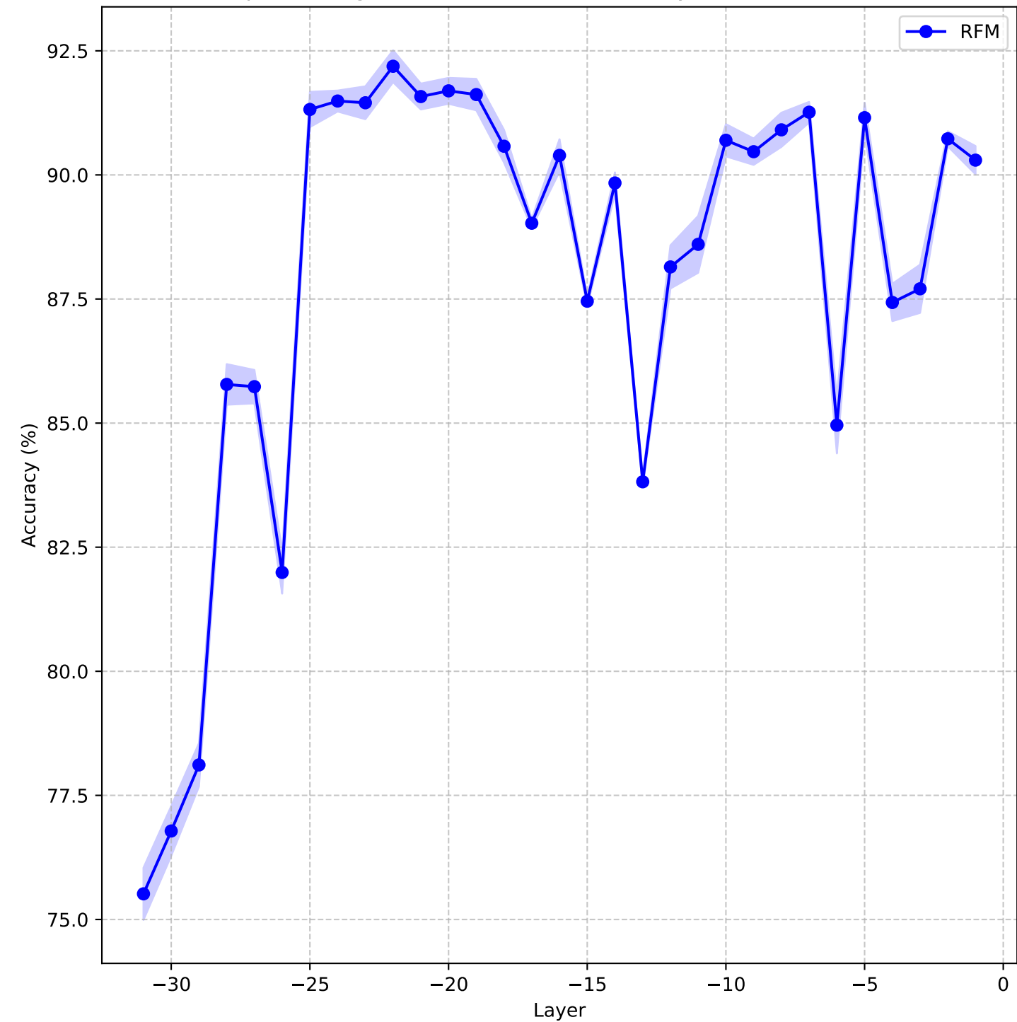
HE (qa), Average Test Accuracies Across Layers for LLama-3-8b-it
