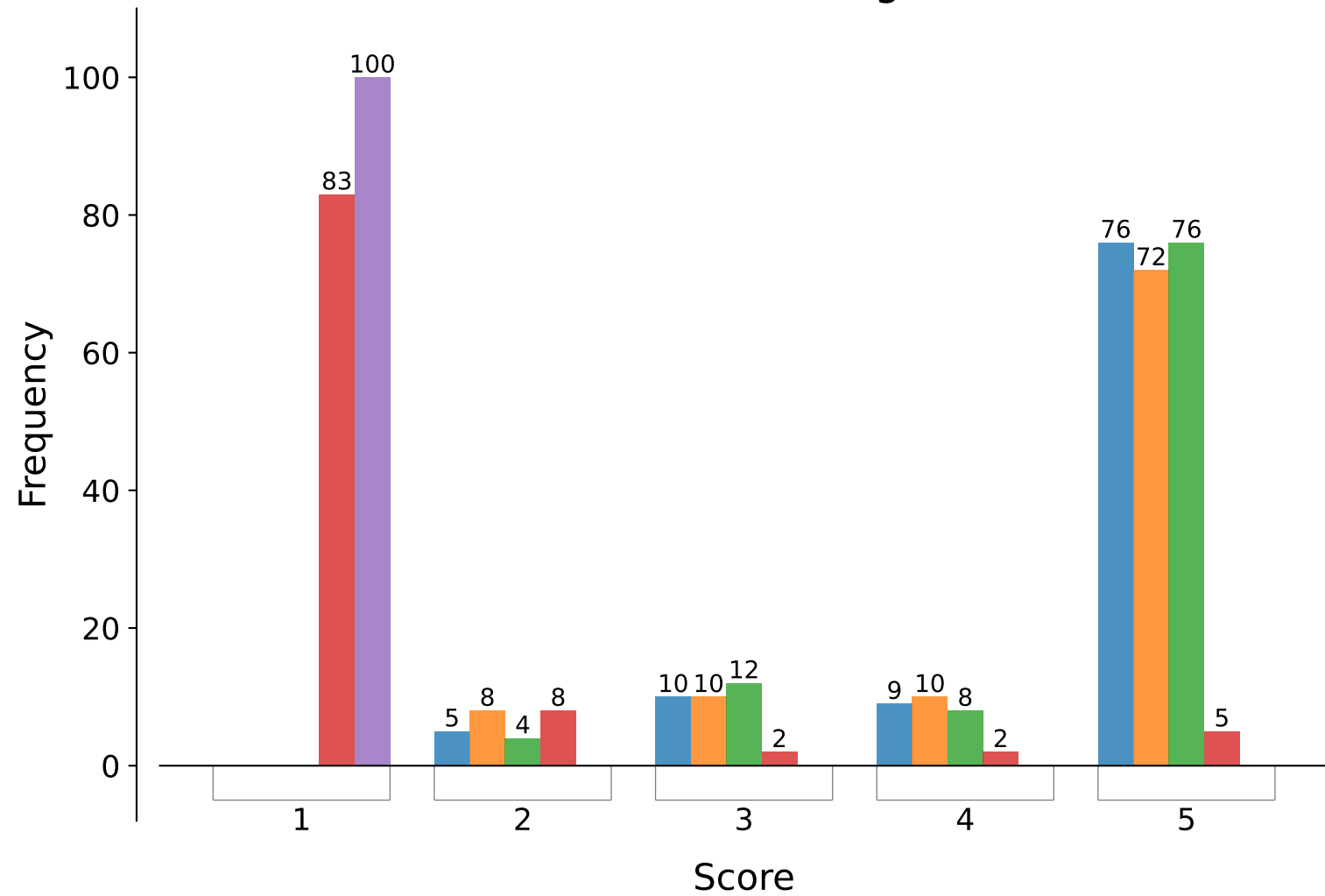
Score Distribution for gemma-2
