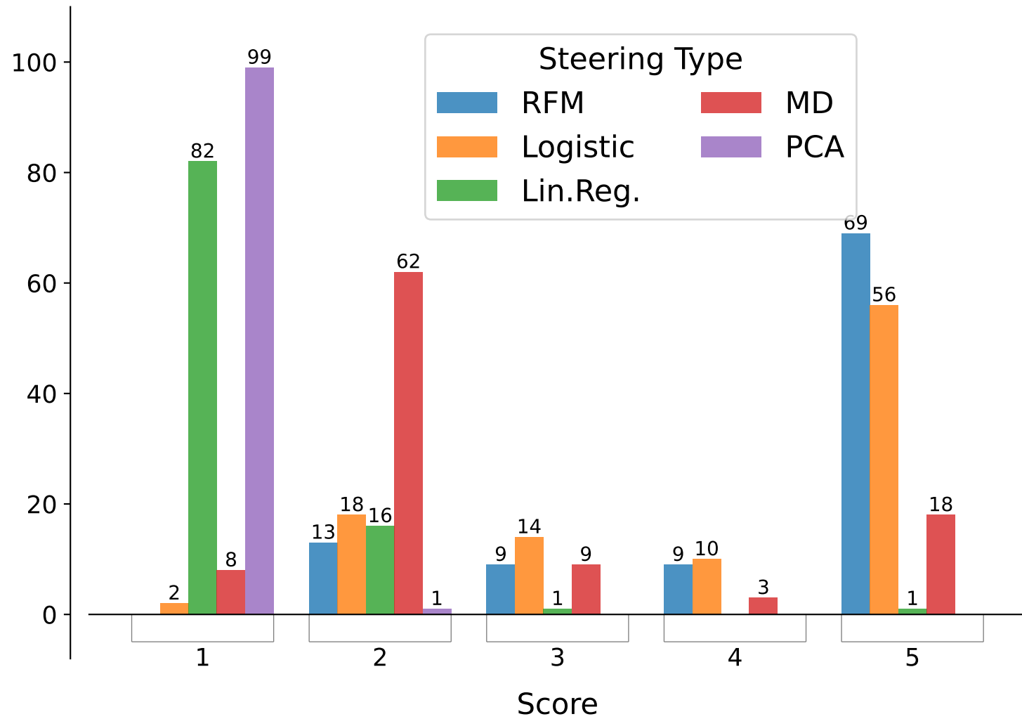
Score Distribution for llama-3
