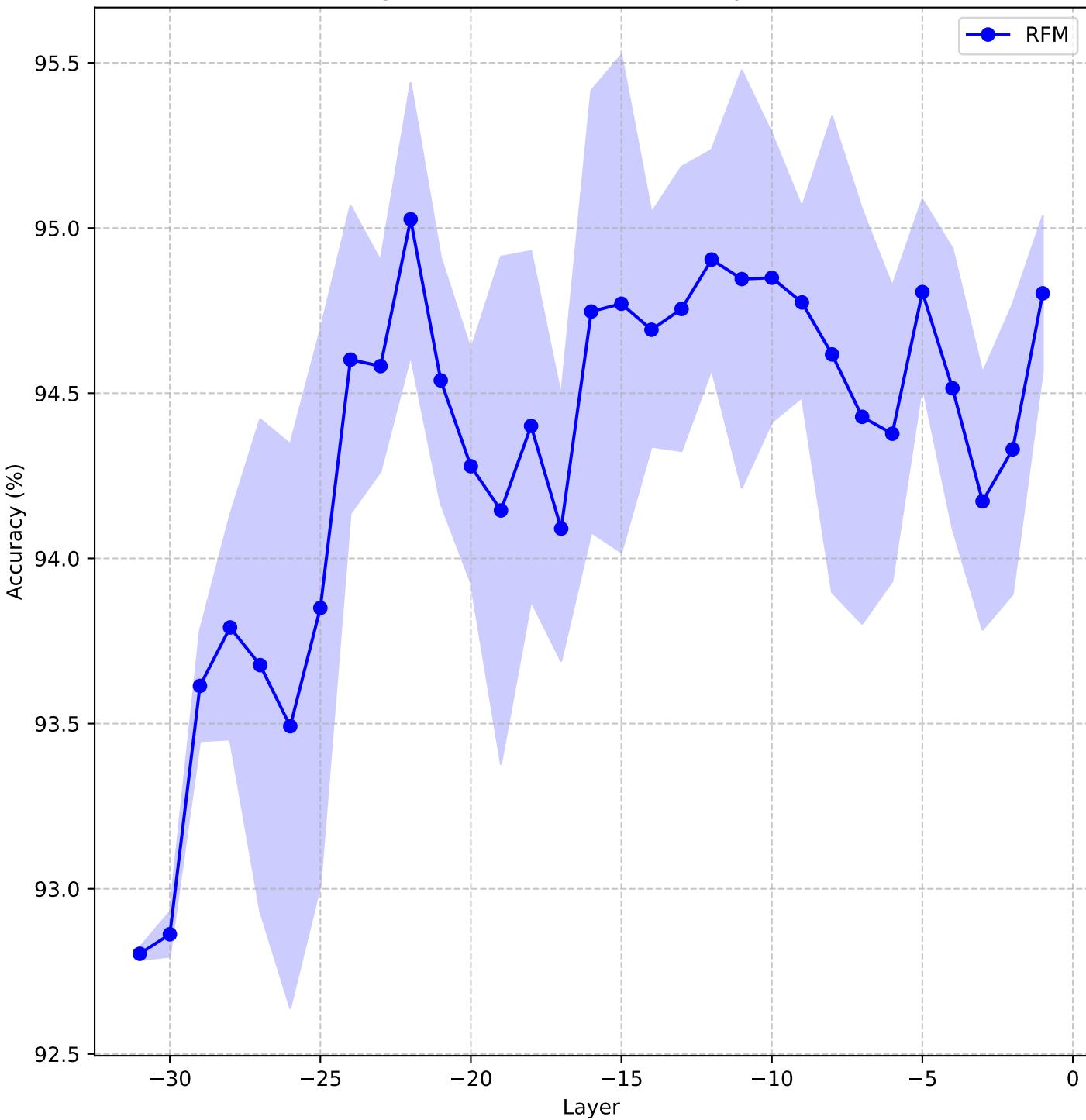
ToxicChat, Average Test Accuracies Across Layers for Llama-3-8b-it
