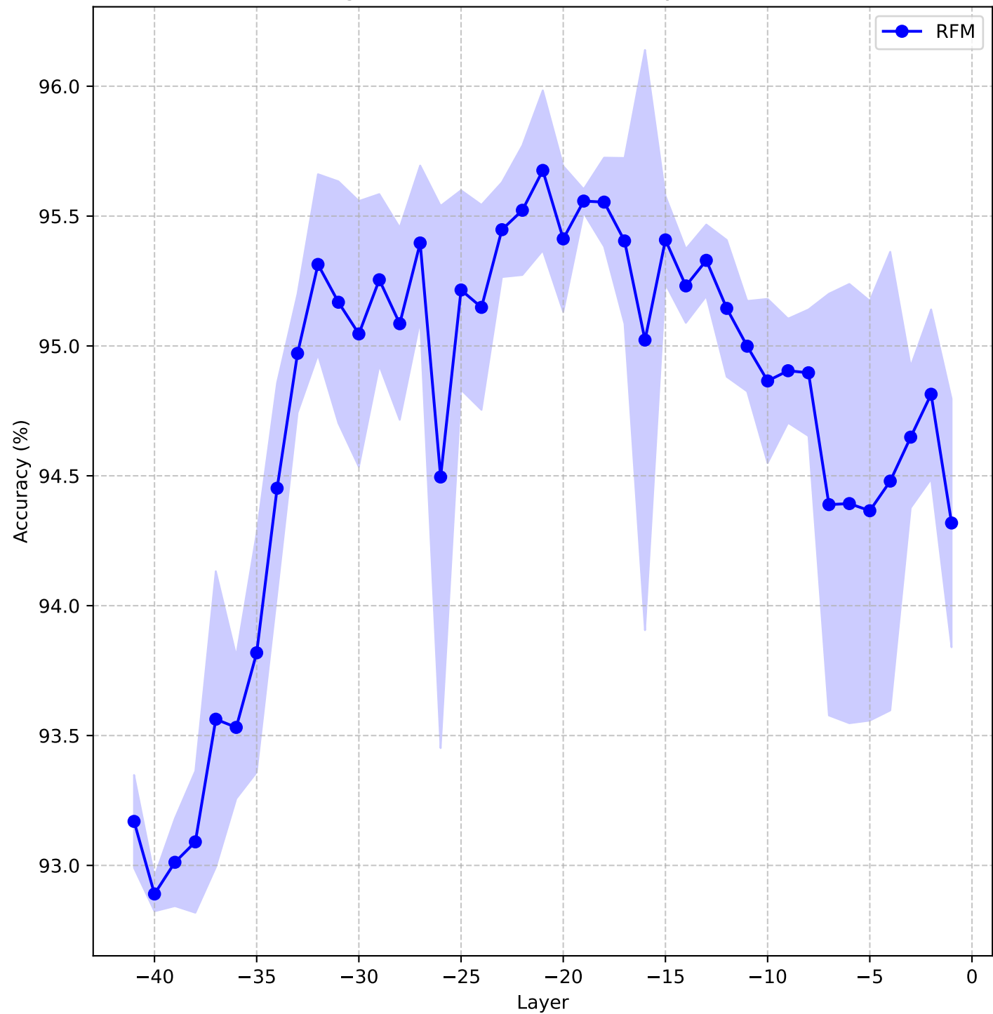
ToxicChat, Average Test Accuracies Across Layers for Gemma-2-9b-it
