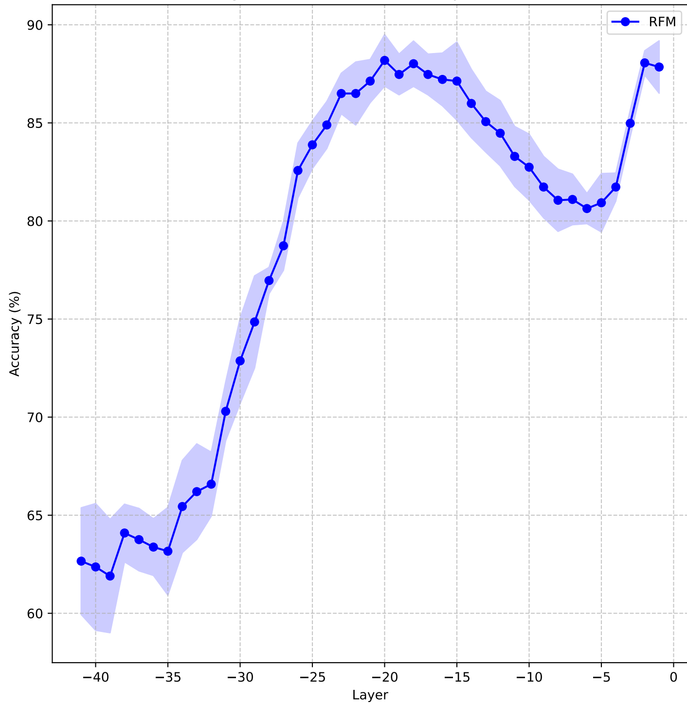
TruthGen, Average Test Accuracies Across Layers for Gemma-2-9b-it
