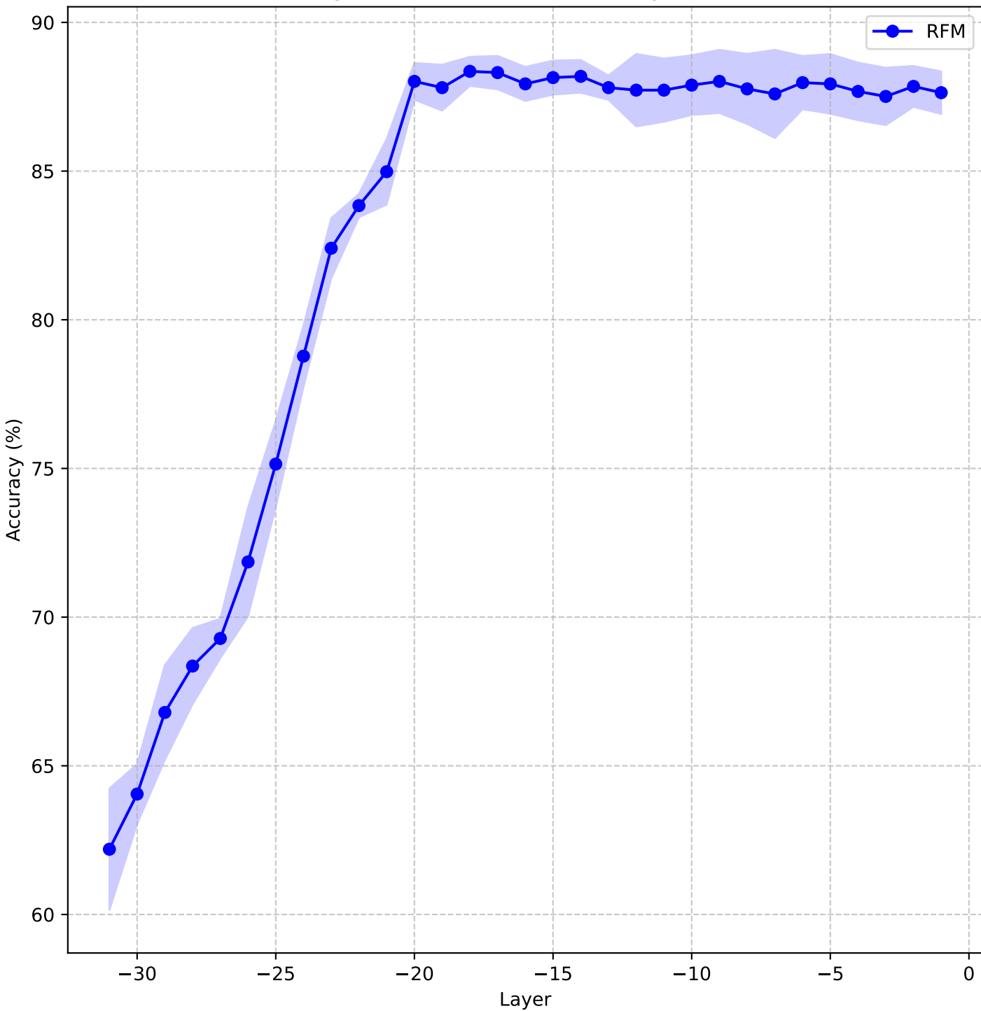
TruthGen, Average Test Accuracies Across Layers for LLama-3-8b-it
