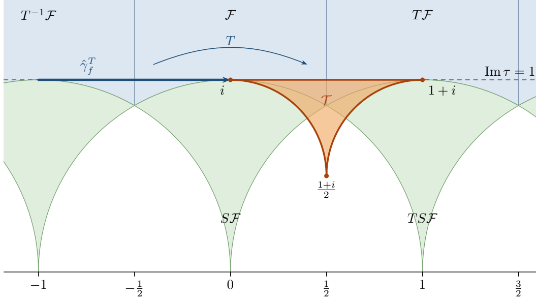
Figure 1: The region \mathcal{T} of Definition 4.21, shaded, with \partial\mathcal{T} in bold. The reference segment \hat{\gamma}_f^T runs from i-1 to i (arrowed): \mathcal{T} is capped not by \hat{\gamma}_f^T itself but by its translate T\hat{\gamma}_f^T , and the two lower arcs are UT\hat{\gamma}_f^T and U^2T\hat{\gamma}_f^T = S^{-1}\hat{\gamma}_f^T , tangent to one another at \frac{1+i}{2} . So \partial\mathcal{T} is the U -orbit of T\hat{\gamma}_f^T , and \mathcal{T} is U -invariant. Superimposed are the fundamental domain \mathcal{F} , its image S\mathcal{F} under S : \tau \mapsto -1/\tau , and the T -translates of both. Note that \mathcal{T} is contained in none of them: it is cut by \operatorname{Re} \tau = \frac{1}{2} and by the arcs |\tau| = 1 and |\tau - 1| = 1 , so it meets \mathcal{F} , T\mathcal{F} , S\mathcal{F} and TS\mathcal{F} alike.
