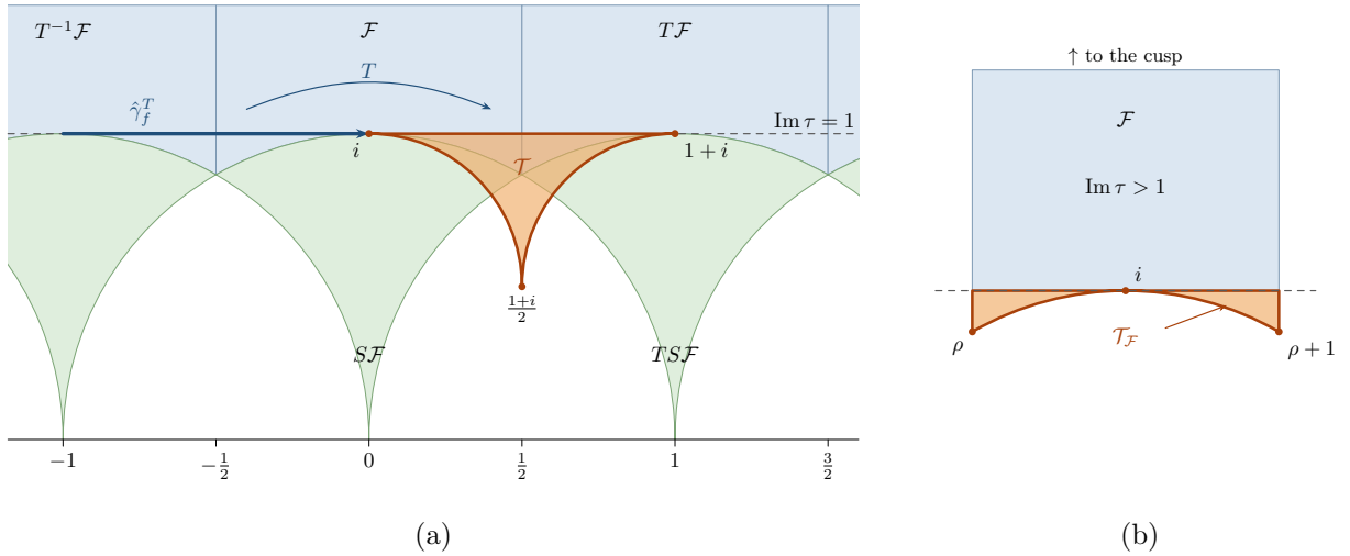
Figure 1: (a) The region \mathcal{T} of Definition 4.21, shaded, boundary in bold. The reference segment \hat{\gamma}_f^T runs from i-1 to i (arrowed): \mathcal{T} is capped not by \hat{\gamma}_f^T itself but by T\hat{\gamma}_f^T , the other two sides being UT\hat{\gamma}_f^T and U^2T\hat{\gamma}_f^T = S^{-1}\hat{\gamma}_f^T , tangent at \frac{1+i}{2} ; so \partial\mathcal{T} is the U -orbit of T\hat{\gamma}_f^T and \mathcal{T} is U -invariant. It lies in no single copy of the fundamental domain, being cut by \operatorname{Re} \tau = \frac{1}{2} and by |\tau| = 1 , |\tau-1| = 1 , and so meets \mathcal{F} , T\mathcal{F} , S\mathcal{F} and TS\mathcal{F} alike. (b) All of \mathcal{T} carried into \mathcal{F} : by (82) the shaded \mathcal{T}_{\mathcal{F}} is the sliver \{\tau \in \mathcal{F} : \operatorname{Im} \tau \leq 1\} , of area \frac{\pi}{3} - 1 = \frac{1}{3}\operatorname{area}(\mathcal{T}) , a fraction 1 - 3/\pi \approx 0.045 of \mathcal{F} . Poles are not excluded there; they are the ones carrying the correction Q_f of Lemma 4.26. Note \mathcal{T}_{\mathcal{F}} is twice the part of \mathcal{T} visible inside \mathcal{F} in (a), the T -, S - and TS -parts folding onto \operatorname{Re} \tau < 0 .
