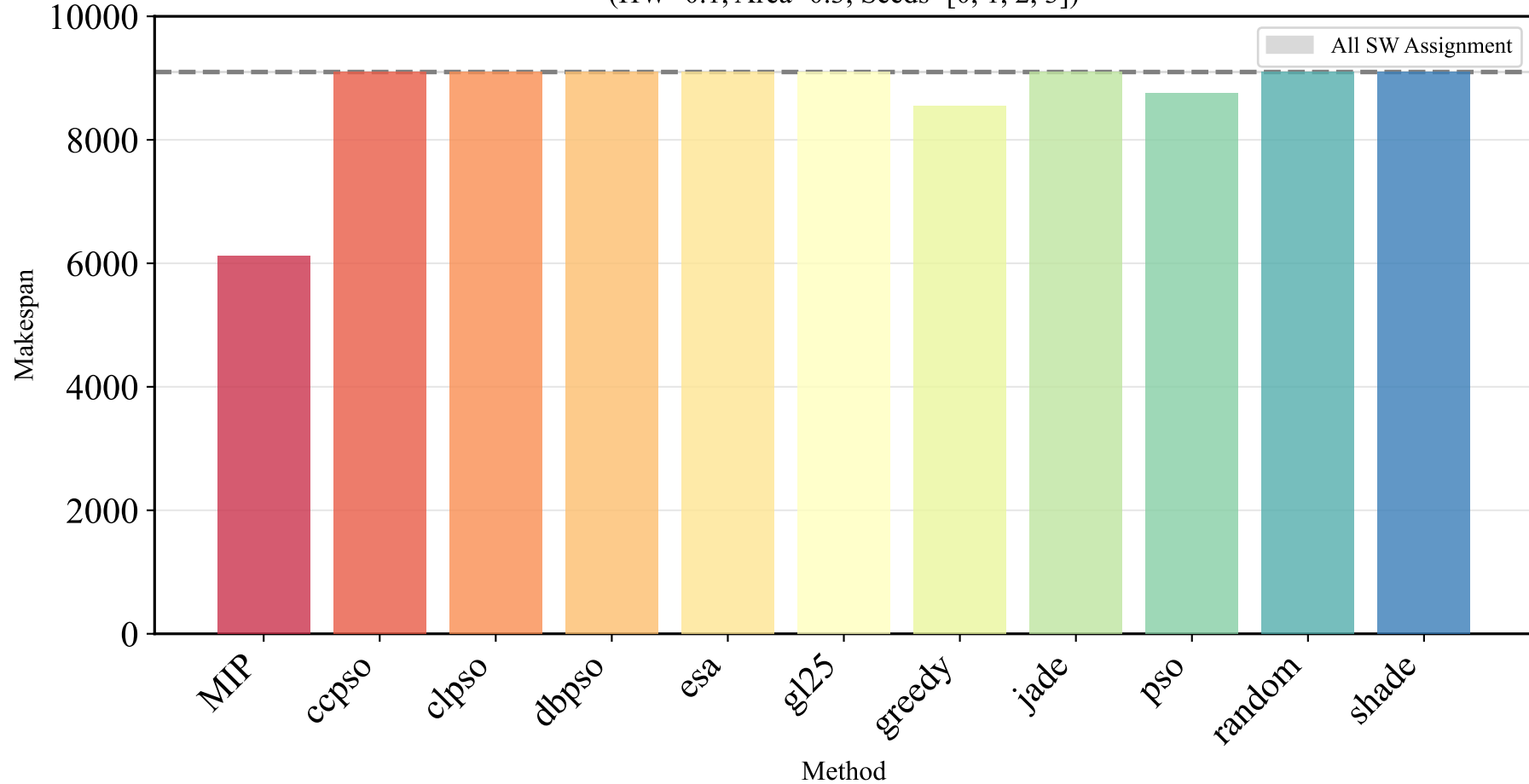
Estimated Optimal Makespan from Partition generated by ARATO Aware Objective Function (HW=0.1, Area=0.3, Seeds=[0, 1, 2, 3])
