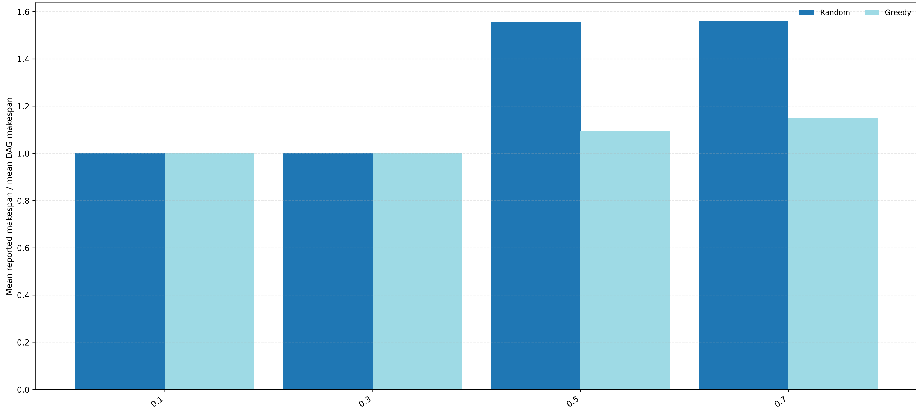
SqueezeNet-TOSA area sweep: mean normalized reported makespan
