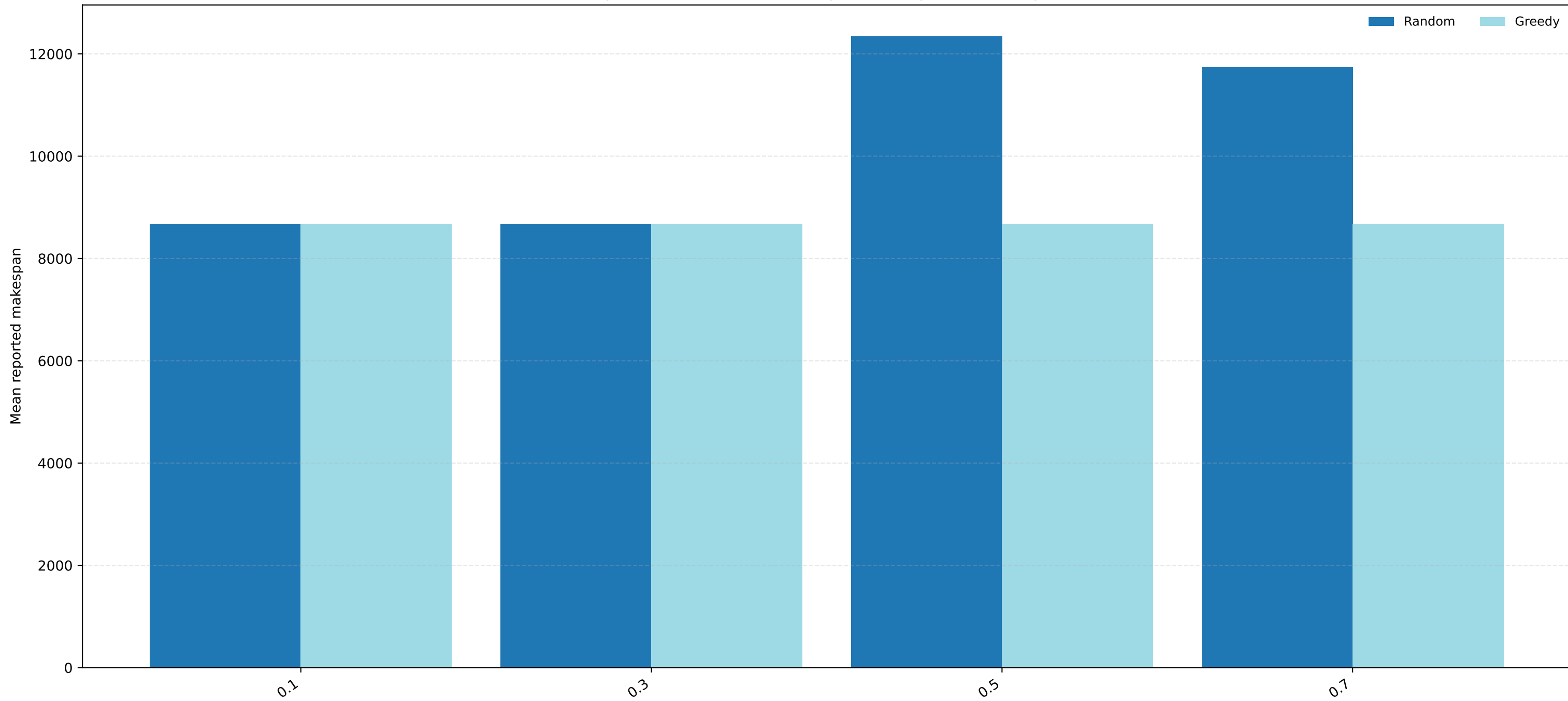
SqueezeNet-TOSA area sweep: mean reported makespan
