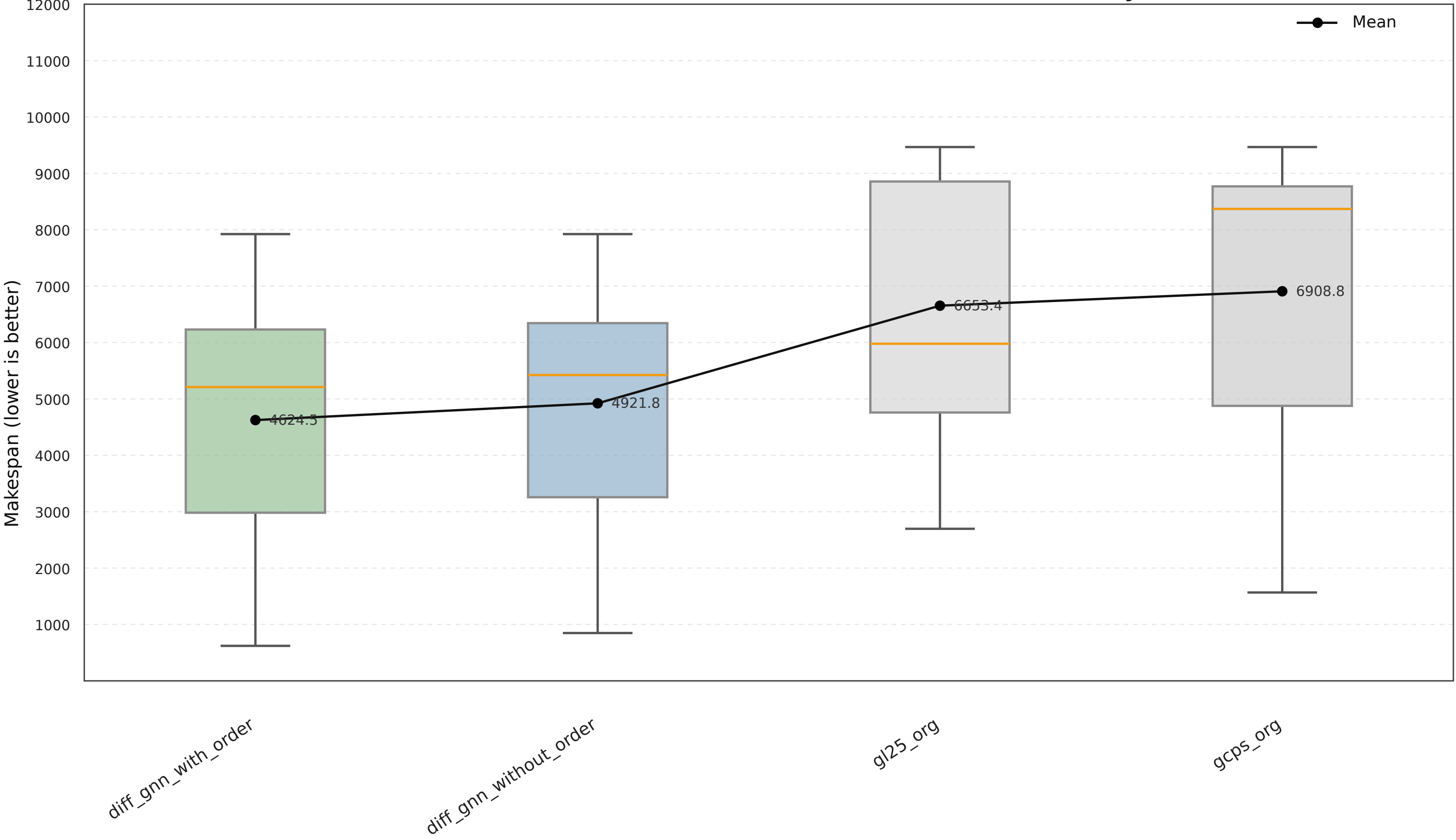
DiffGNN (With/Without Order) vs Baseline Methods (Sorted by Mean)
