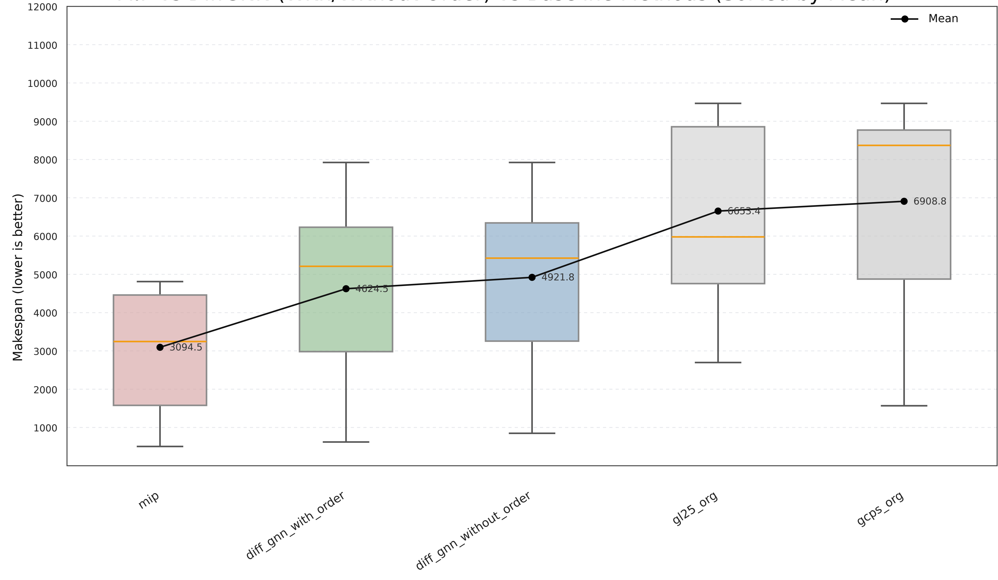
MIP vs DiffGNN (With/Without Order) vs Baseline Methods (Sorted by Mean)
