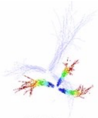
(a) Dataset
