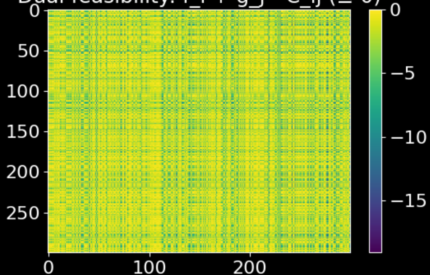
Dual feasibility: f_i + g_j - C_{ij} (\leq 0)
