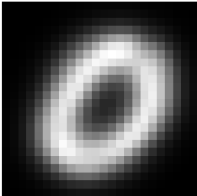
Entropic barycenter reg=1.0
