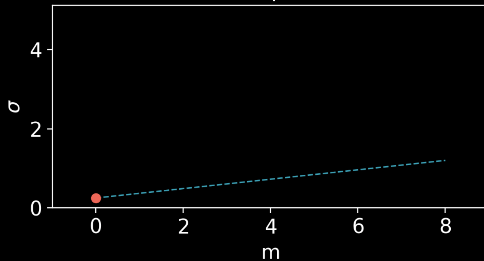
OT Interpolation
