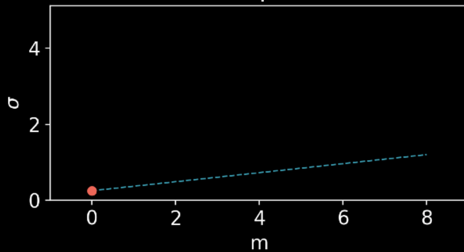
OT Interpolation
