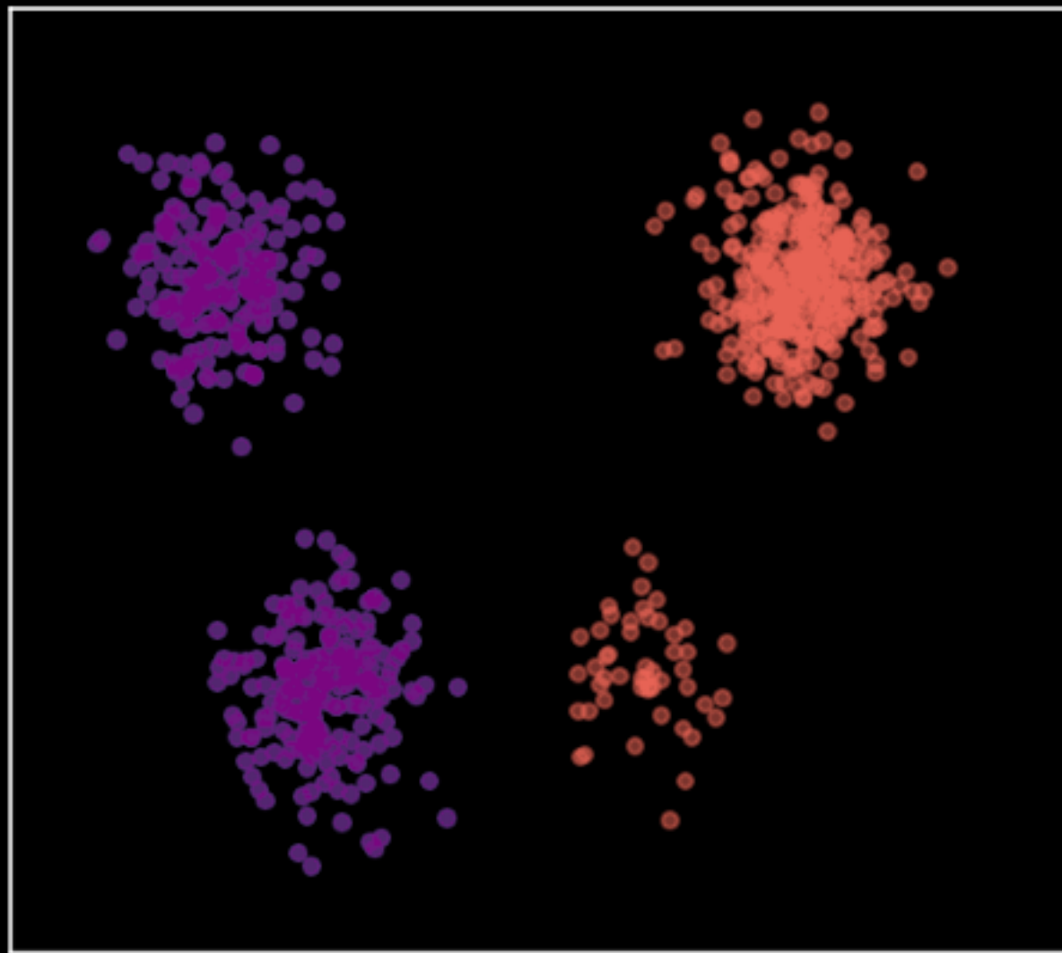
Classical OT ( \tau = +\infty )
