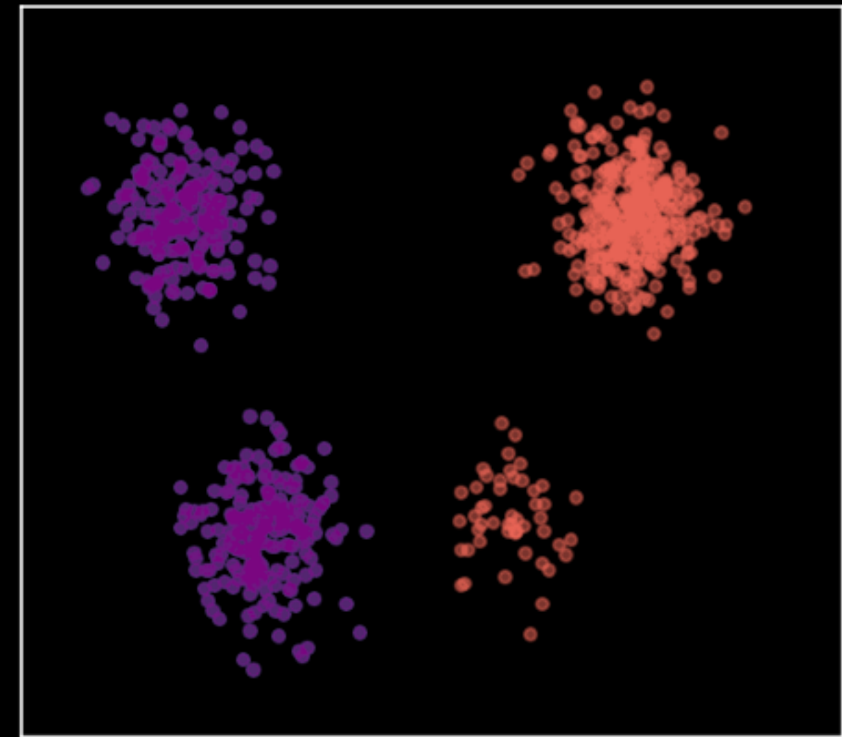
Unbalanced OT ( \tau_a = \tau_b = 0.1 )
