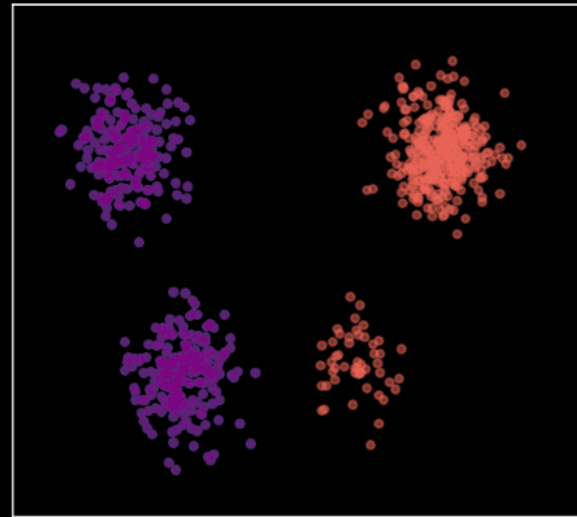
Unbalanced OT ( \tau_b = 0.1 )
