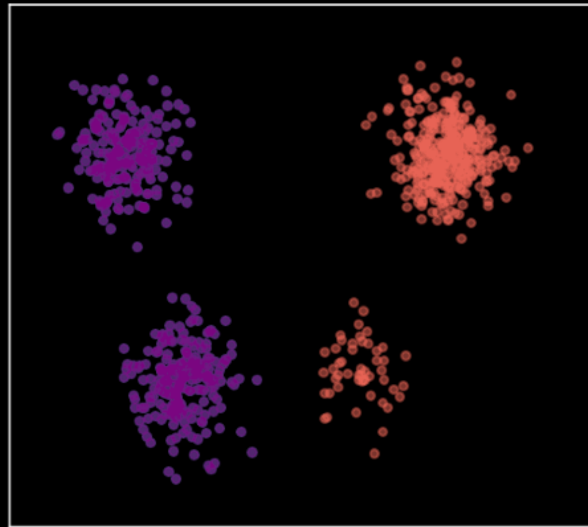
Unbalanced OT ( \tau_a = 0.1 )
