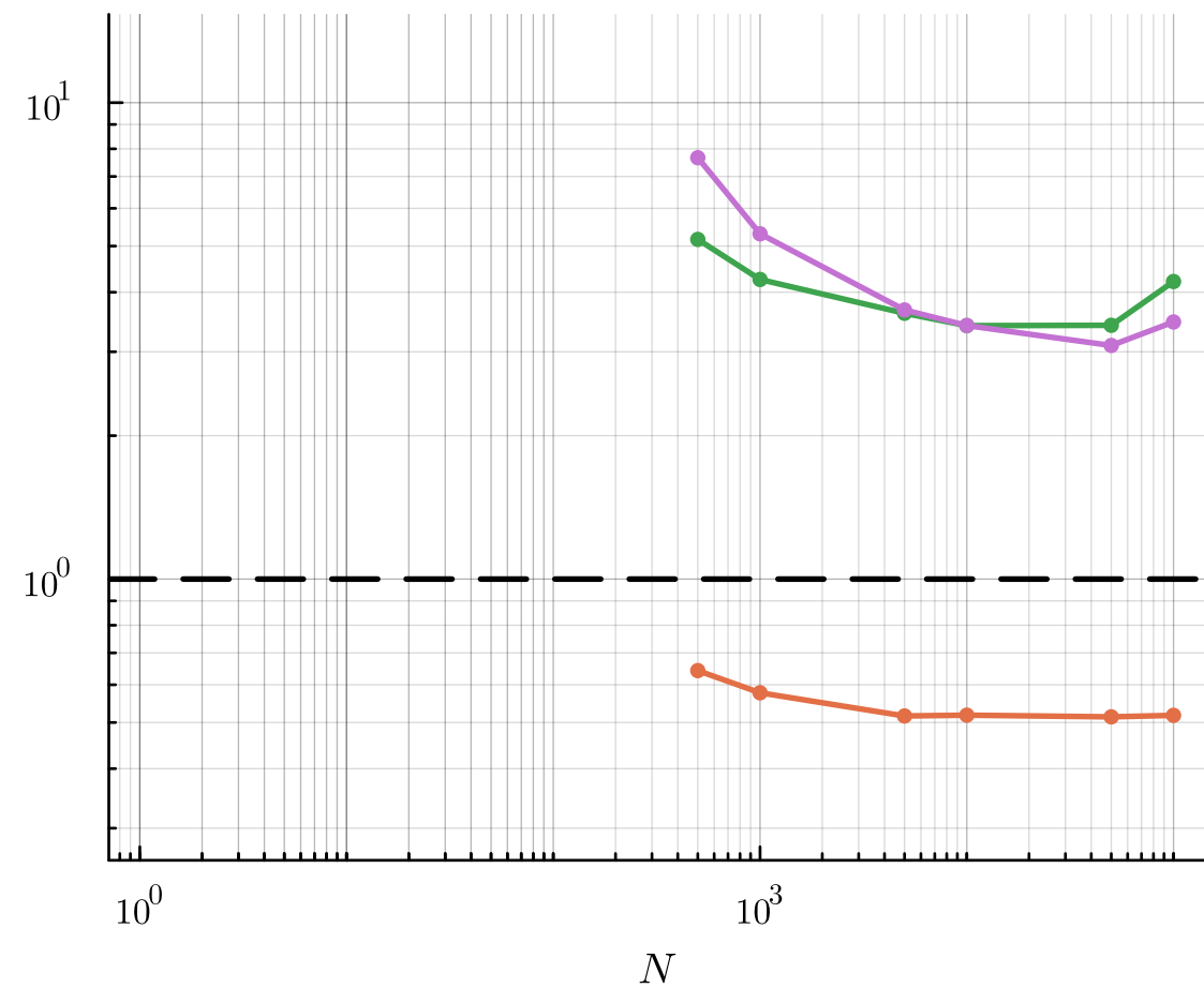
K = 5, D = 1
