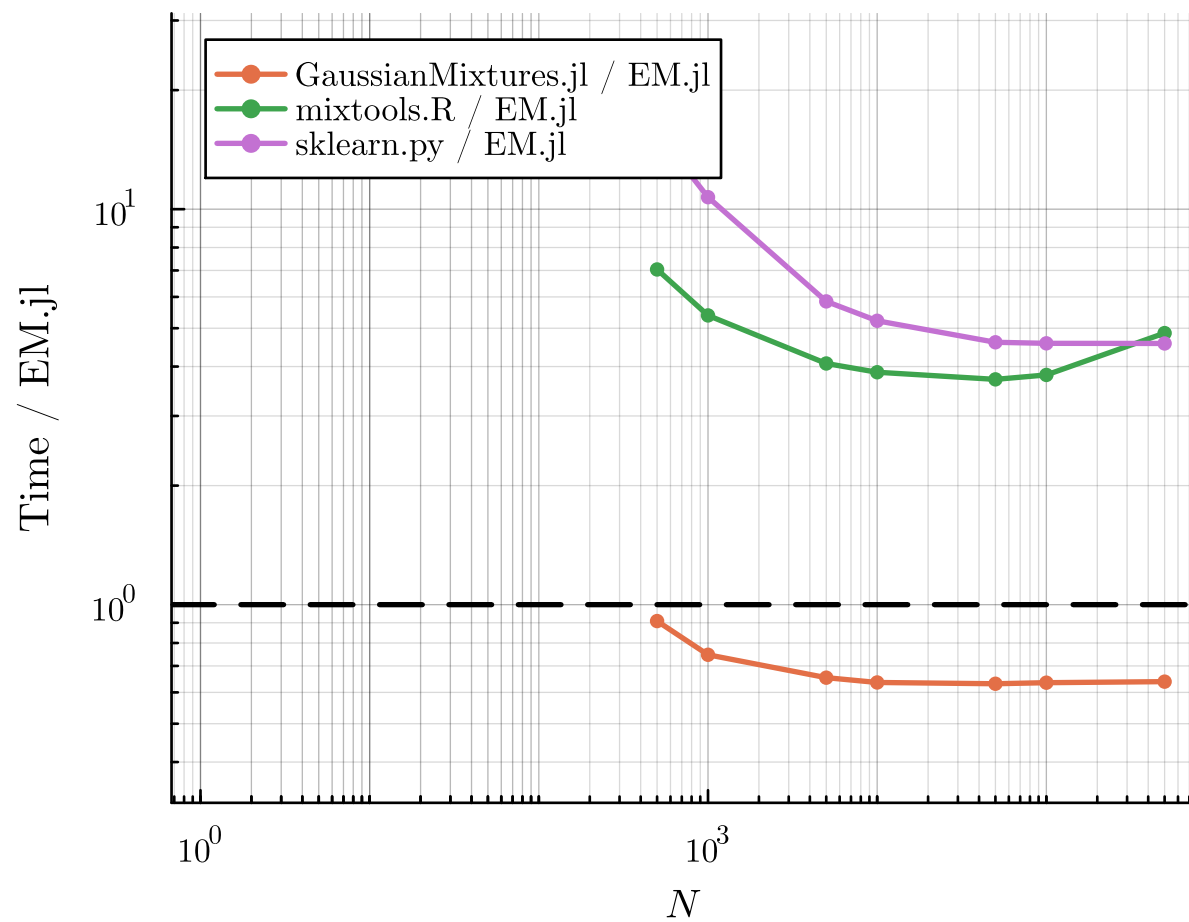
K = 2, D = 1
