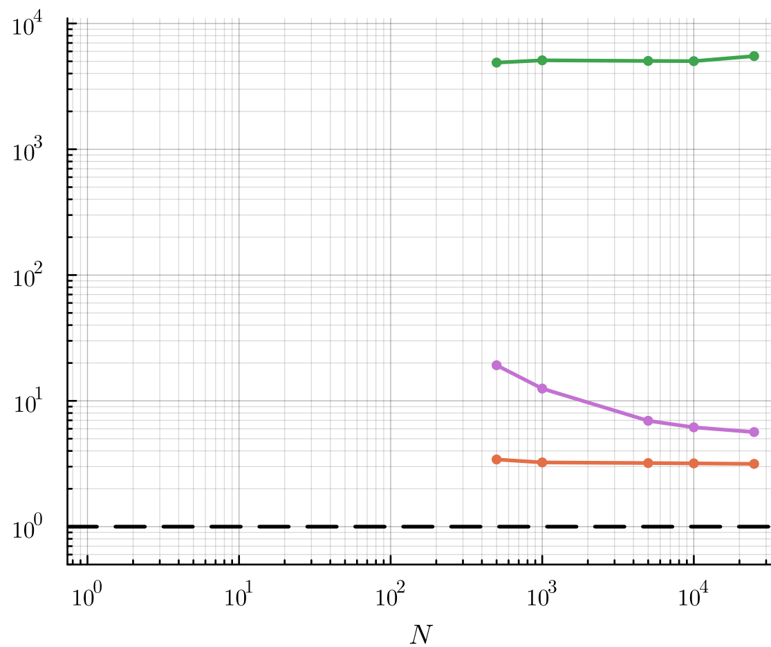
K = 2, D = 2
