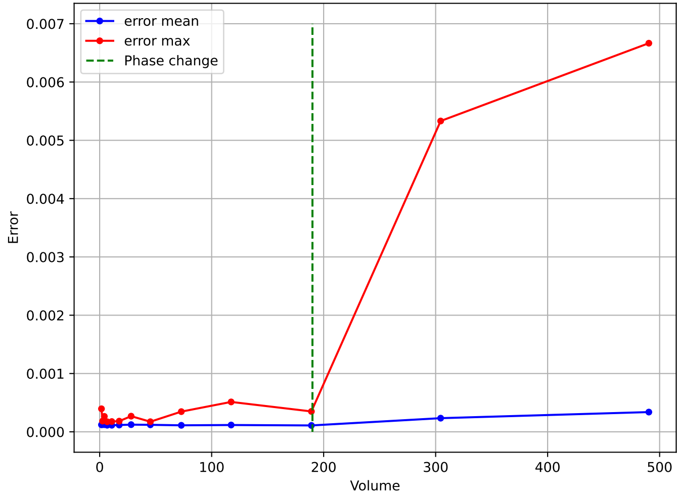
Volume against the batch mean error and batch worst-case error for a stream of + characters - linux x86-64 i5-2520m cpu @ 2.50ghz 4 cores
