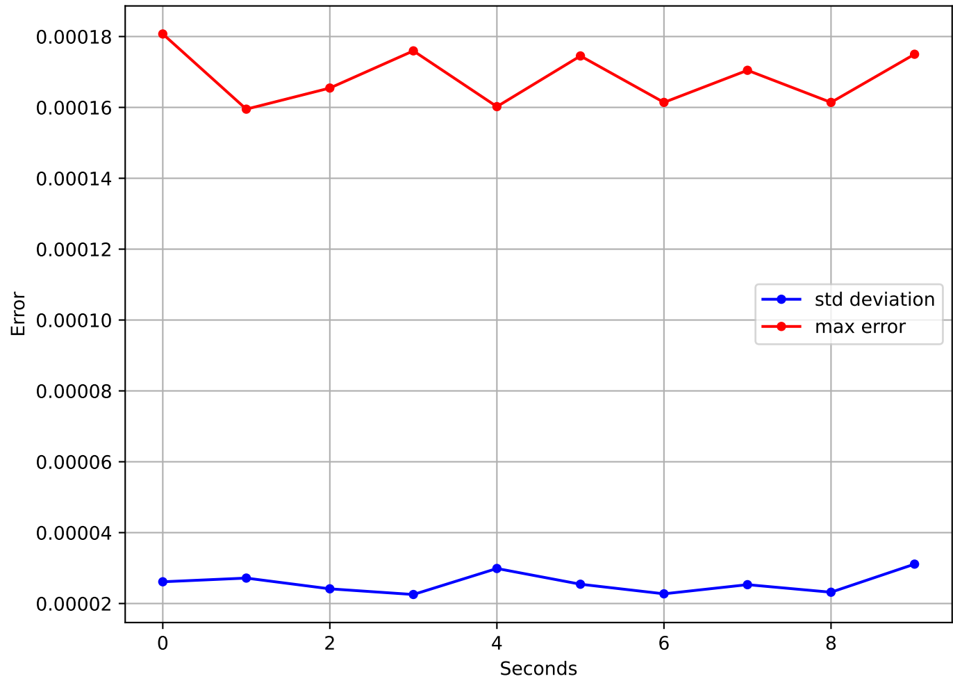
Batch max err & batch std deviation over 10 seconds - linux x86-64 i5-2520m cpu @ 2.50ghz 4 cores
