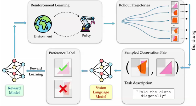
Figure 6: Schematic of using visual language models for rewards for training a policy
