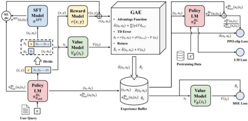
Figure 8: Overall RLHF formulation
