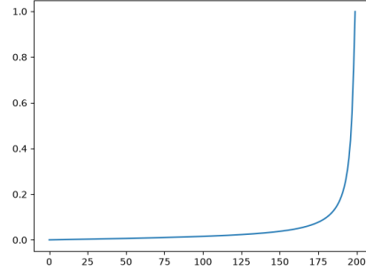
Figure 2: \beta_t for a cosine schedule for t \in [0, 200]
