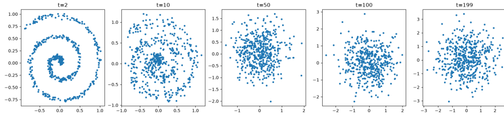
Figure 3: Forward diffusion example
