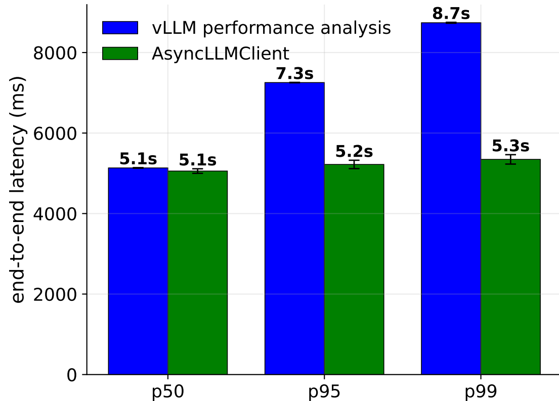
Per-request latency distribution
