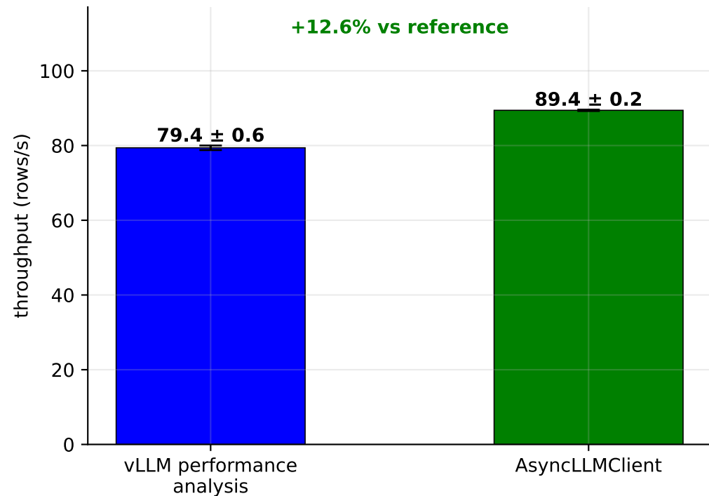
Throughput on vLLM workload
