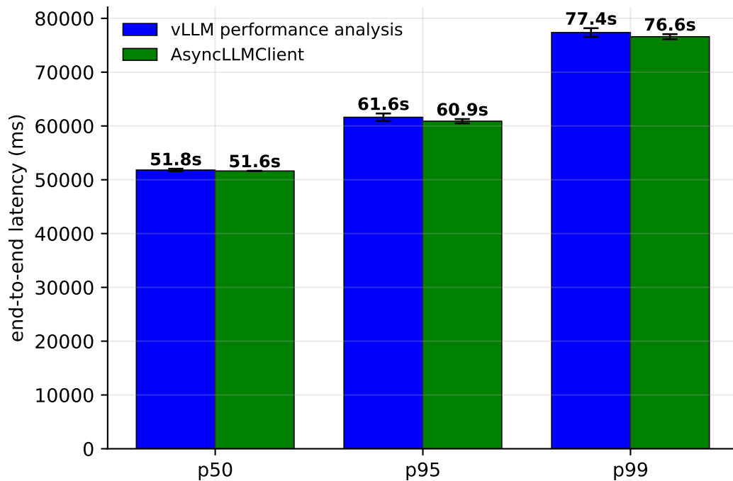
Per-request latency distribution
