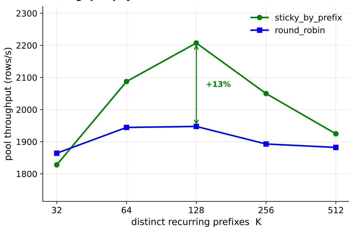
Throughput payoff
