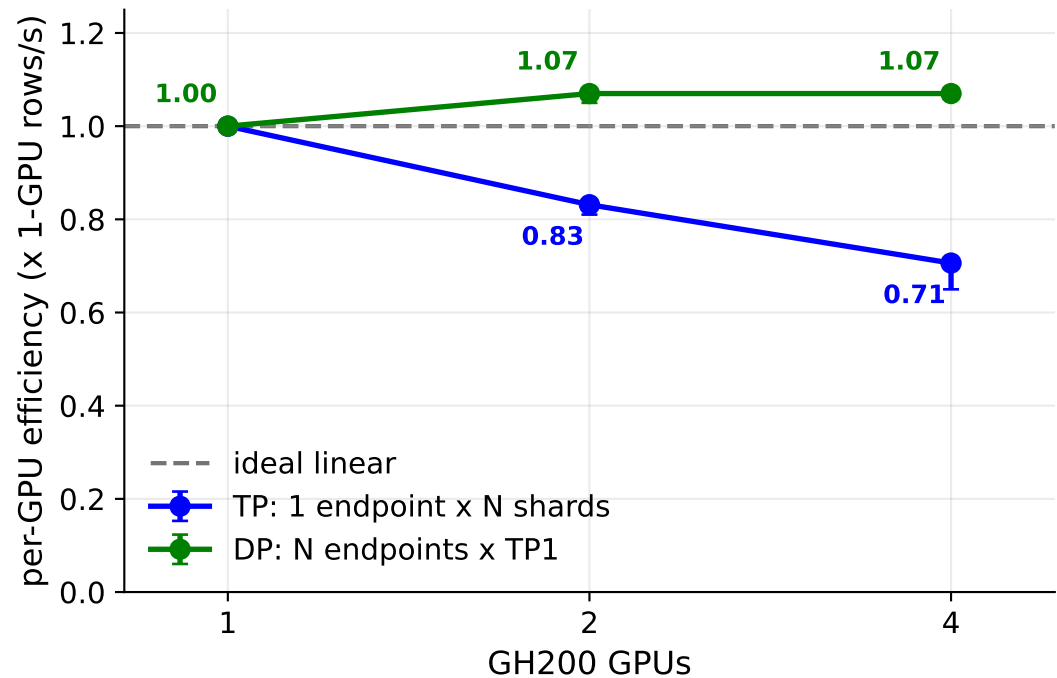
(b) per-GPU efficiency
