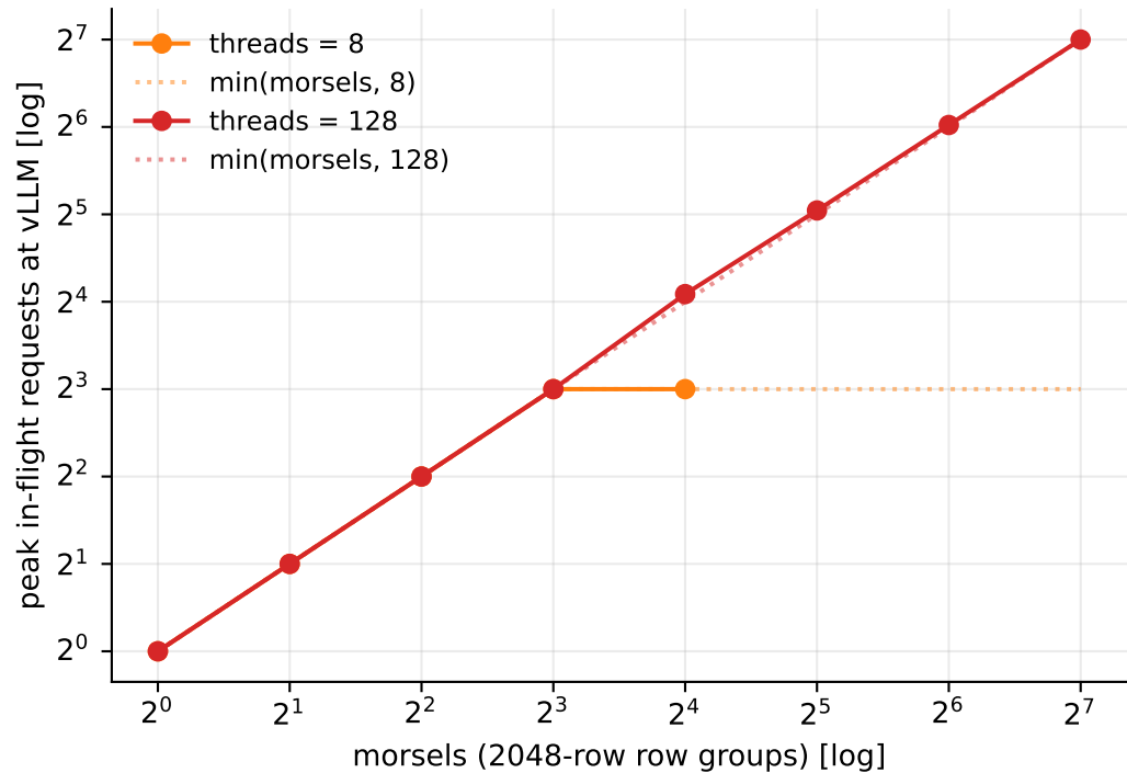
[Morsel sweep] concurrency = \min(\text{morsels}, \text{threads})
