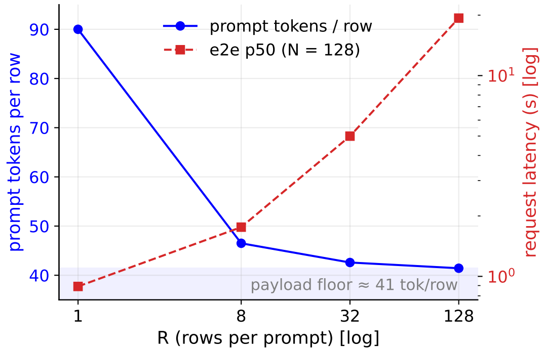
Per-row prompt cost and request latency
