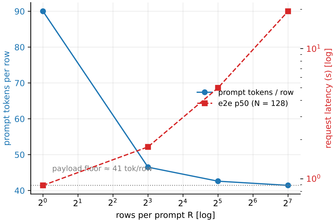
[The trade] template amortised by R = 32 ; latency keeps growing
