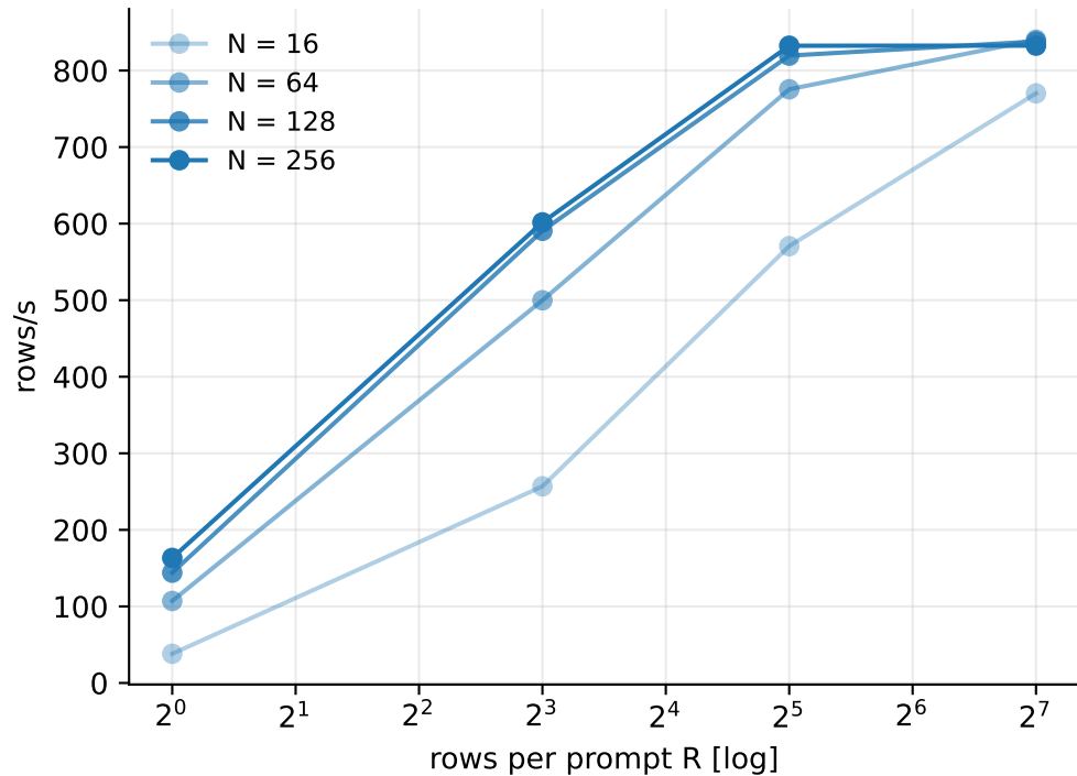
[Row packing] R amortises prefill; flat past R = 32
