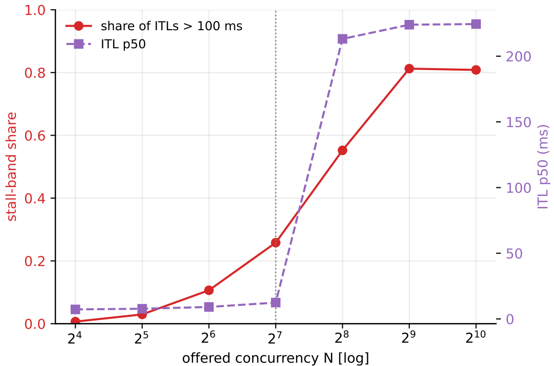
[The cliff] the median crosses between N=128 and N=256
