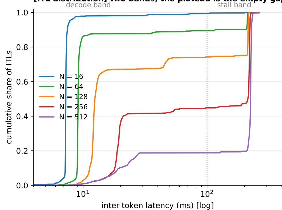
[ITL distribution] two bands; the plateau is the empty gap
