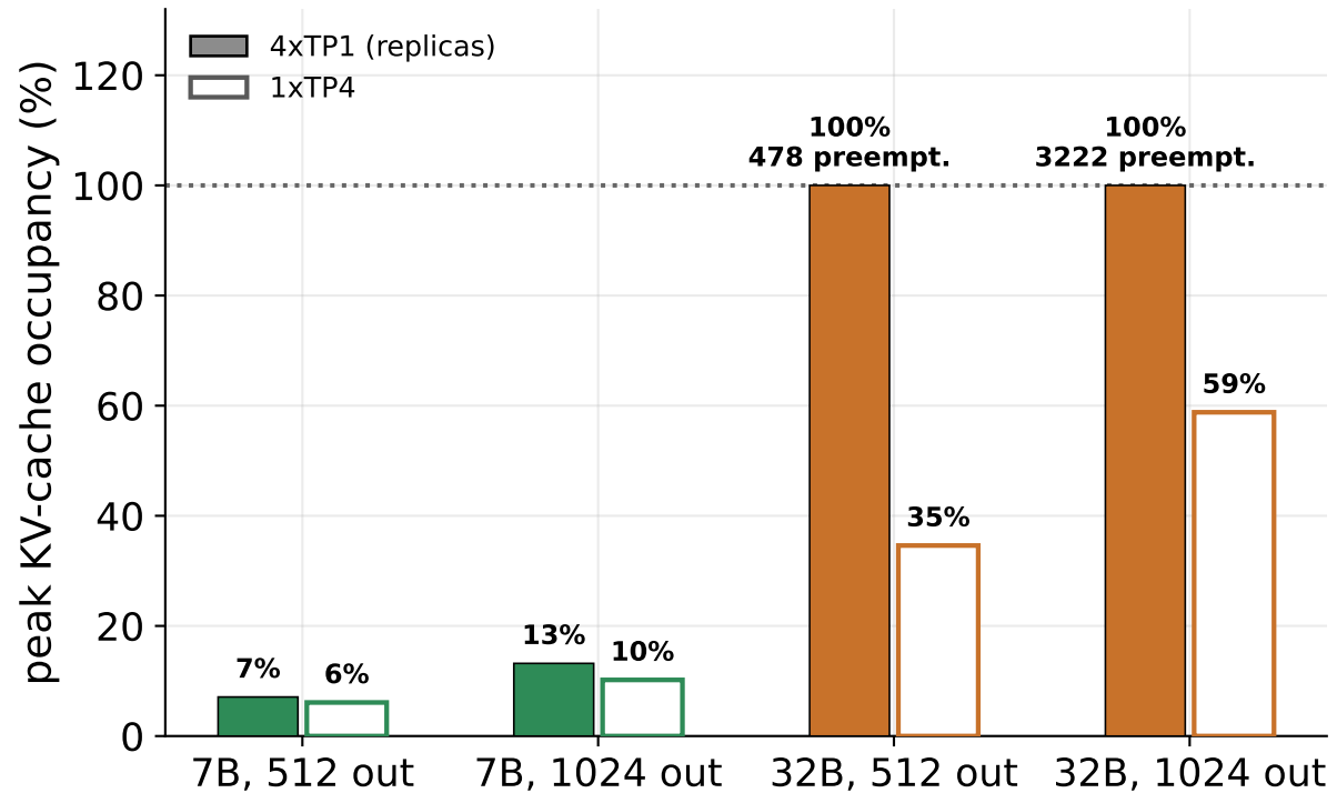
KV pressure
