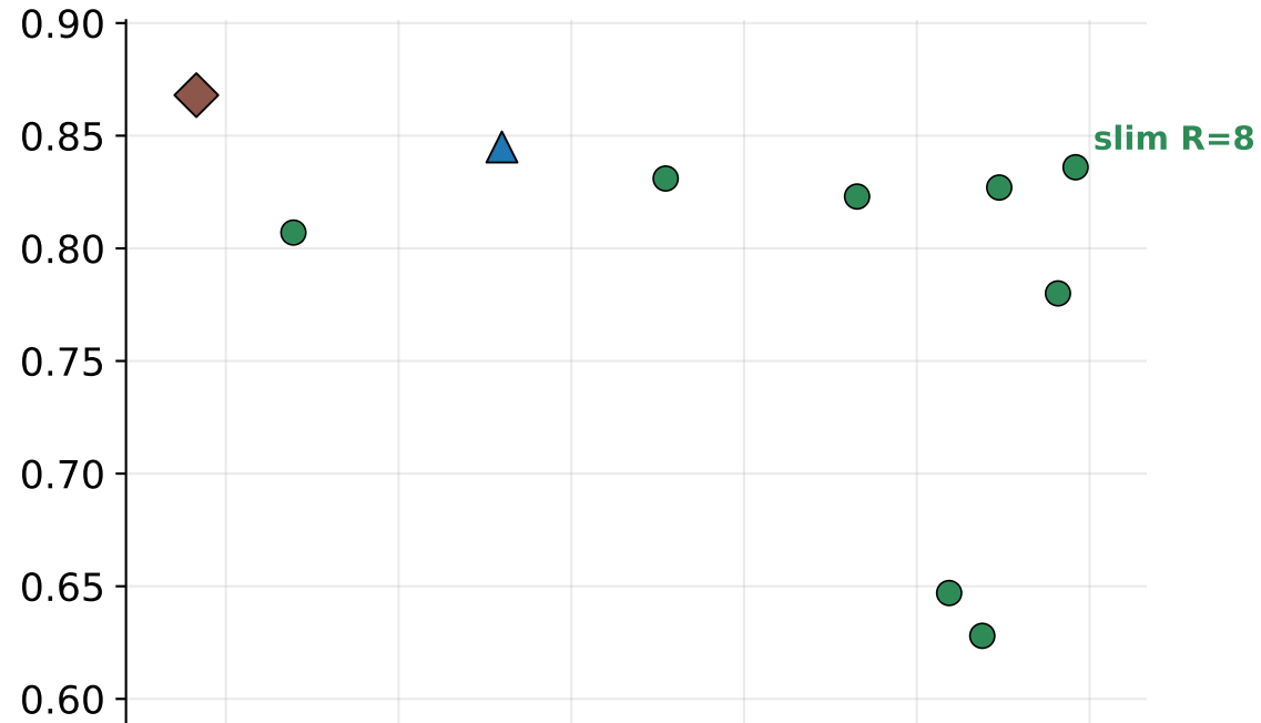
Qwen2.5-7B — extract
