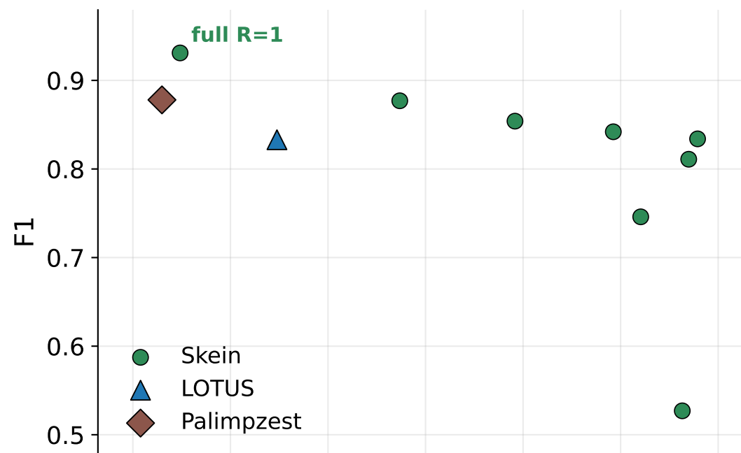
Qwen2.5-7B — filter
