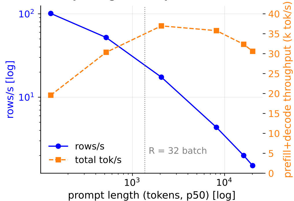
Prompt-length sweep
