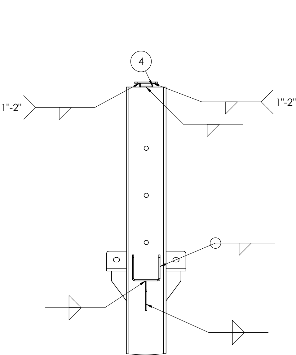
DETAIL A SCALE 1 : 12
