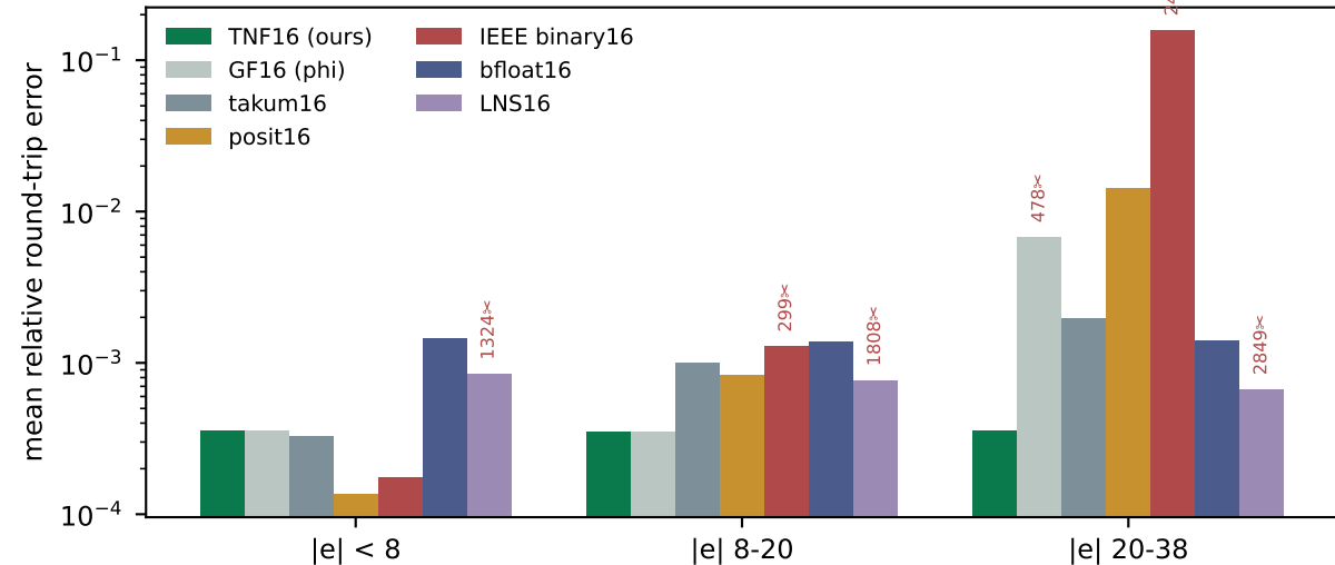
16-bit-class formats on one workload ( \infty = values that overflowed)
