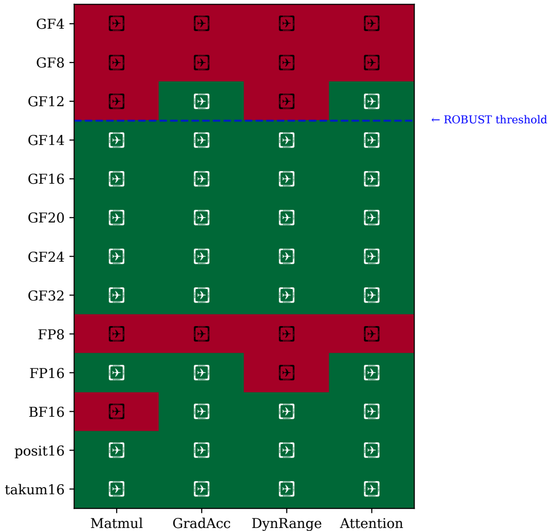
ML Workload Robustness Matrix
