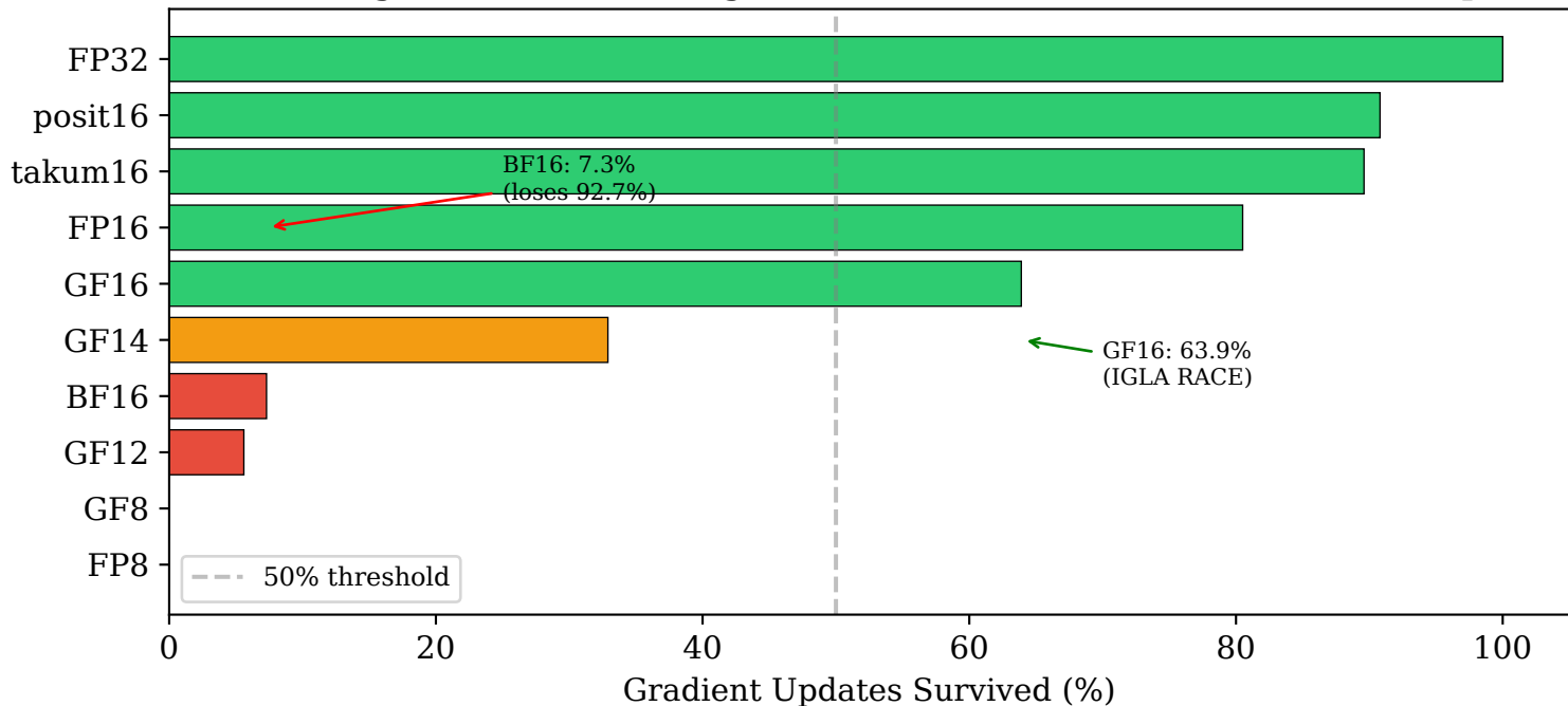
Training Noise Floor: Weight = 0.5 \pm N(0.0001, 0.001) , 2000 steps
