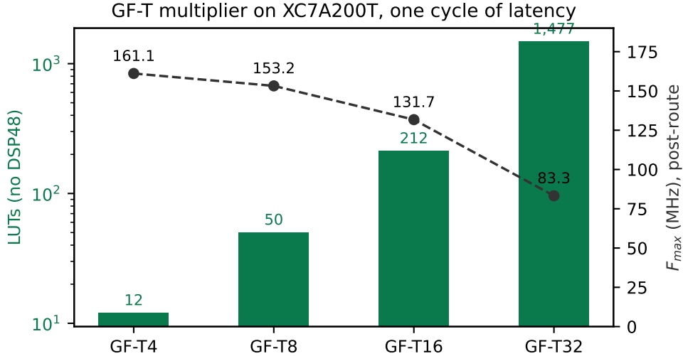
Figure 2: Area and achieved frequency across the ladder.
