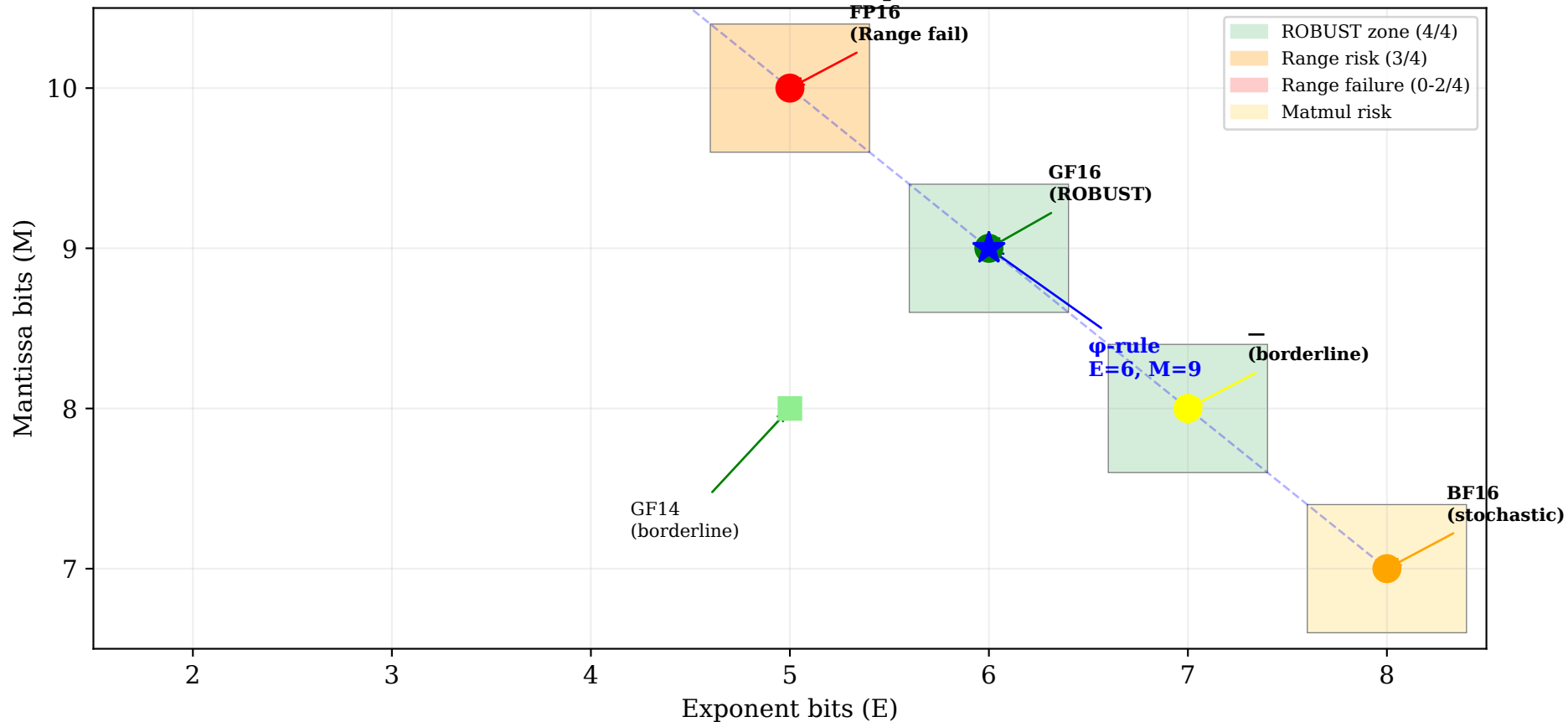
16-bit Format Failure Mode Map (W=16, M=15-E)
