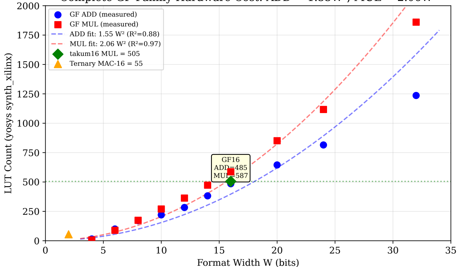
Complete GF Family Hardware Cost: \text{ADD} = 1.55W^2 , \text{MUL} = 2.06W^2
