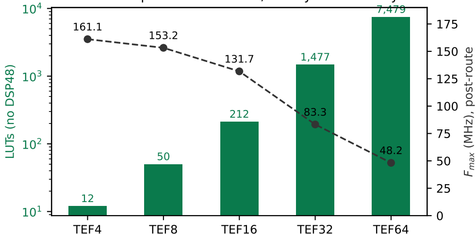
TEF multiplier on XC7A200T, one cycle of latency
