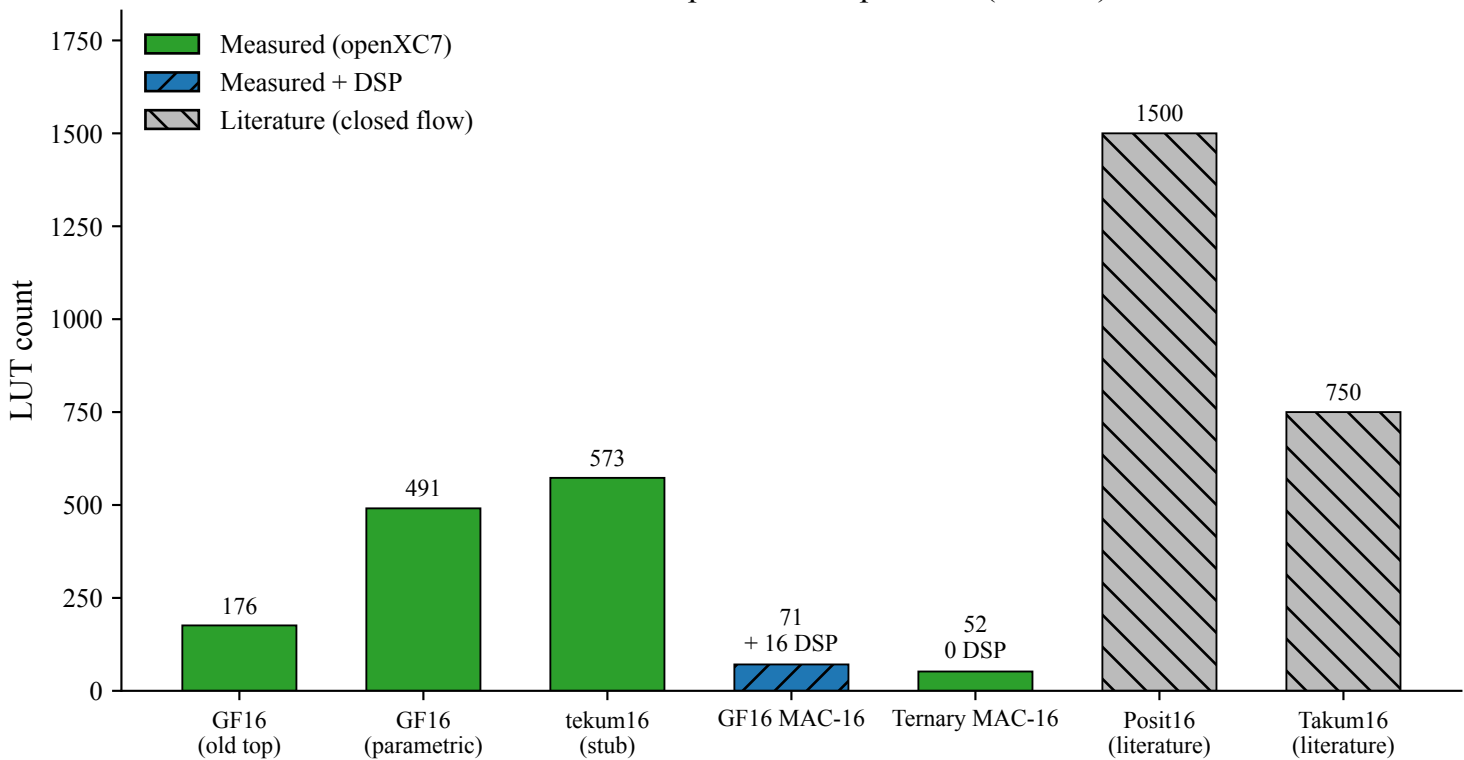
LUT Cost Comparison on openXC7 (Artix-7)
