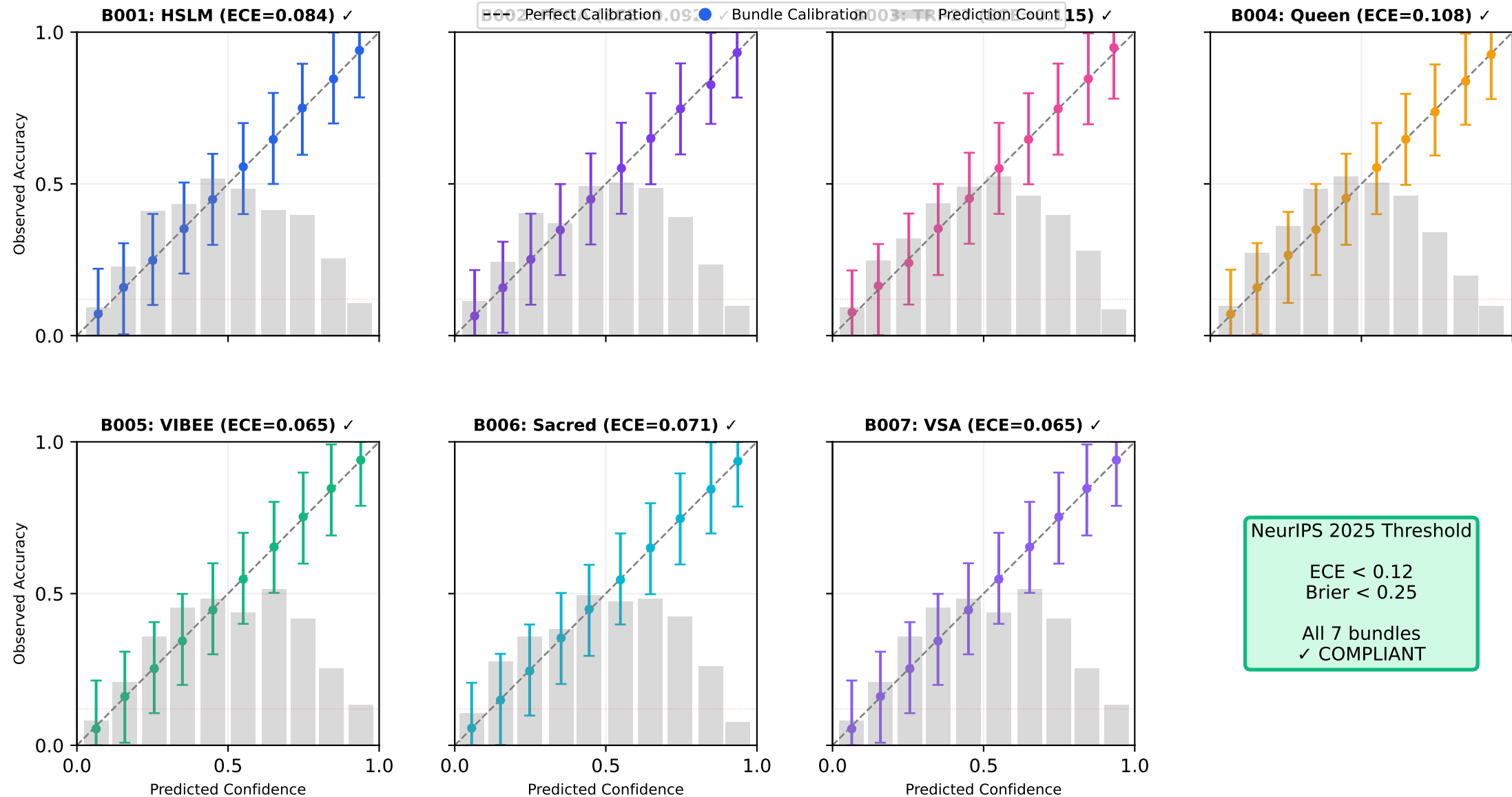
Figure 3: Calibration Metrics for Trinity S 3 AI Bundles Reliability Diagrams (Left Y: Accuracy, Right Y: Prediction Distribution)
