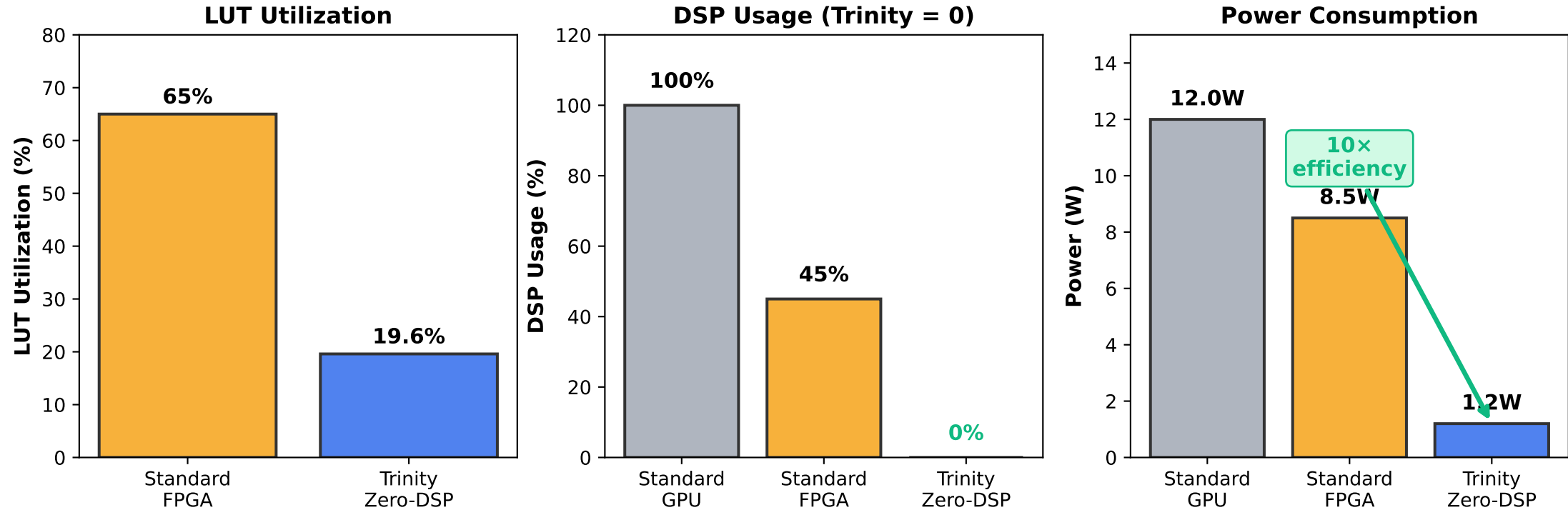
Figure 4: FPGA Resource Utilization Comparison
