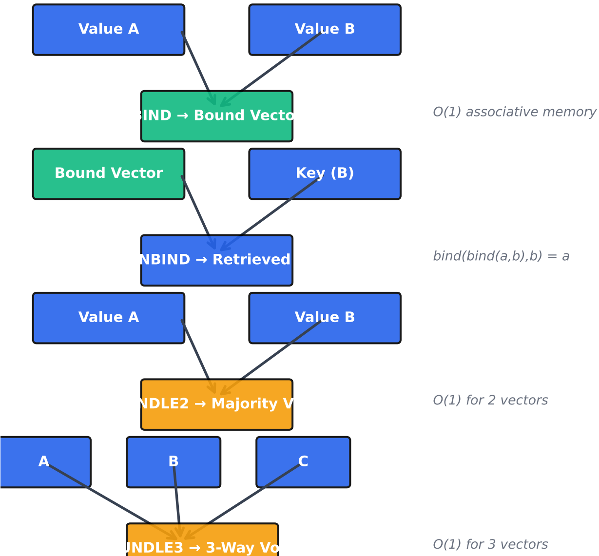
Figure 5: Vector Symbolic Architecture (VSA) Operations
