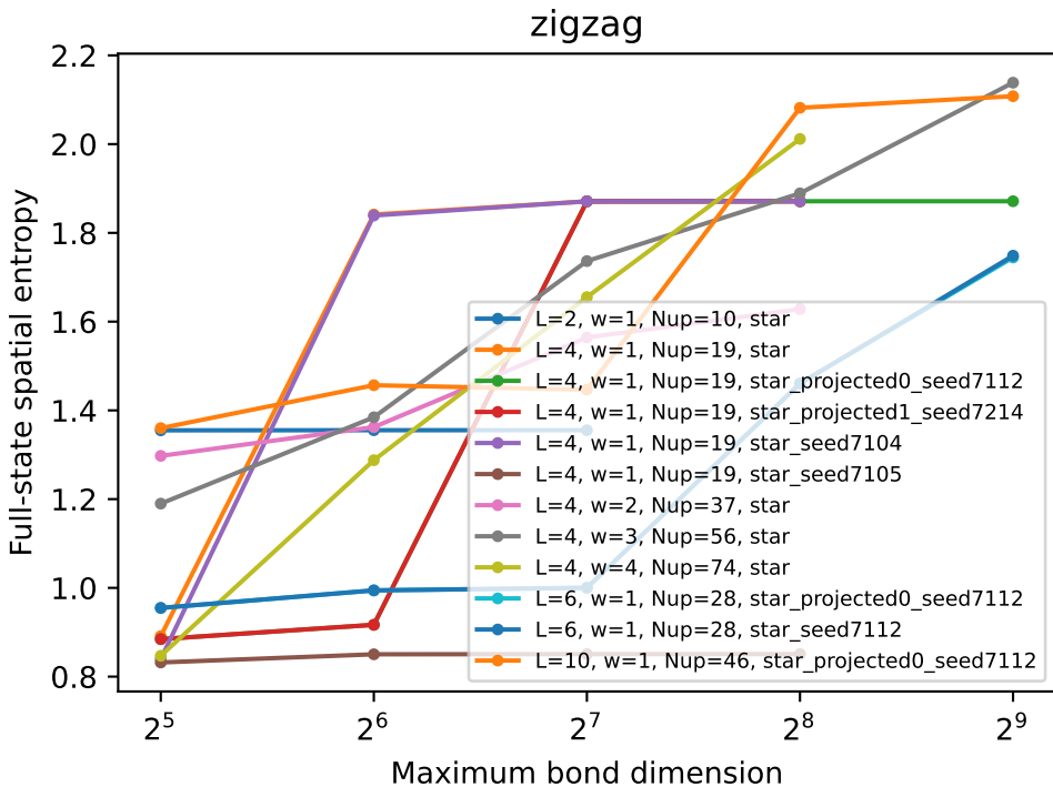
Bond dependence within separate initialization and number branches
