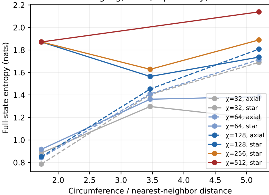
zigzag; L=4 (exploratory)
