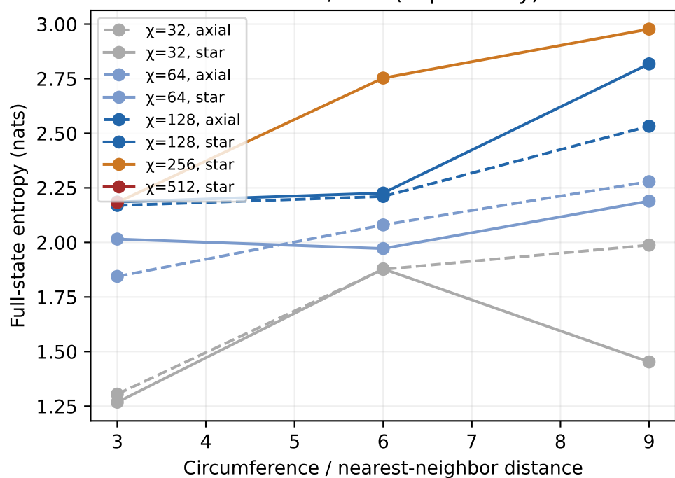
armchair; L=4 (exploratory)
