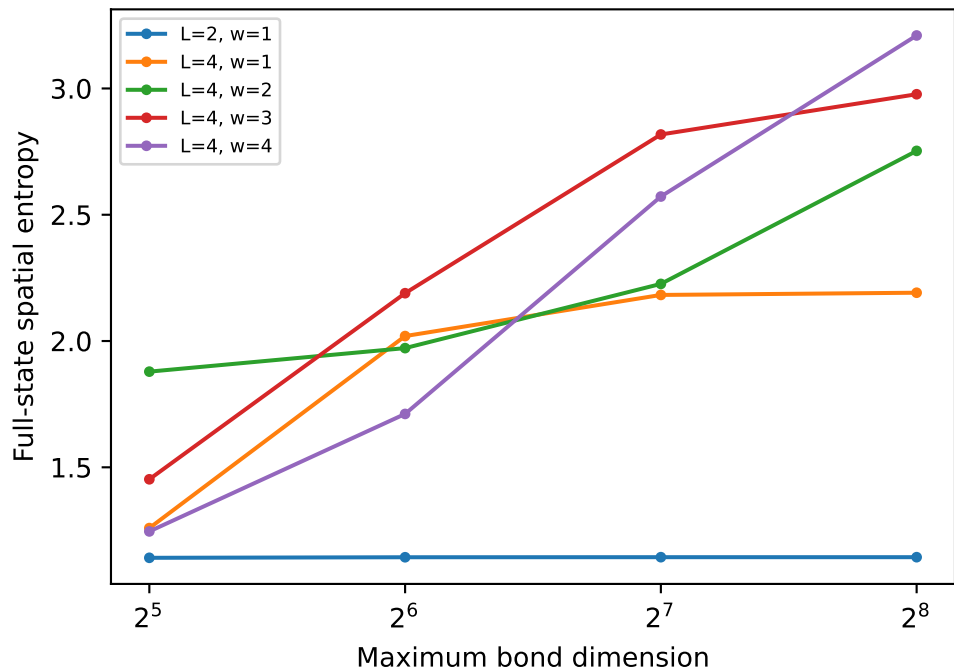
Bond-dimension dependence (lowest recorded energy per seed comparison)
