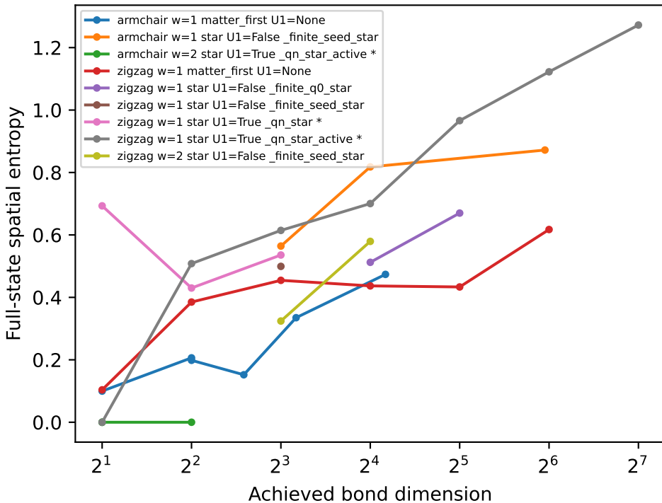
Separate infinite variational branches; * includes energy above a trial bound
