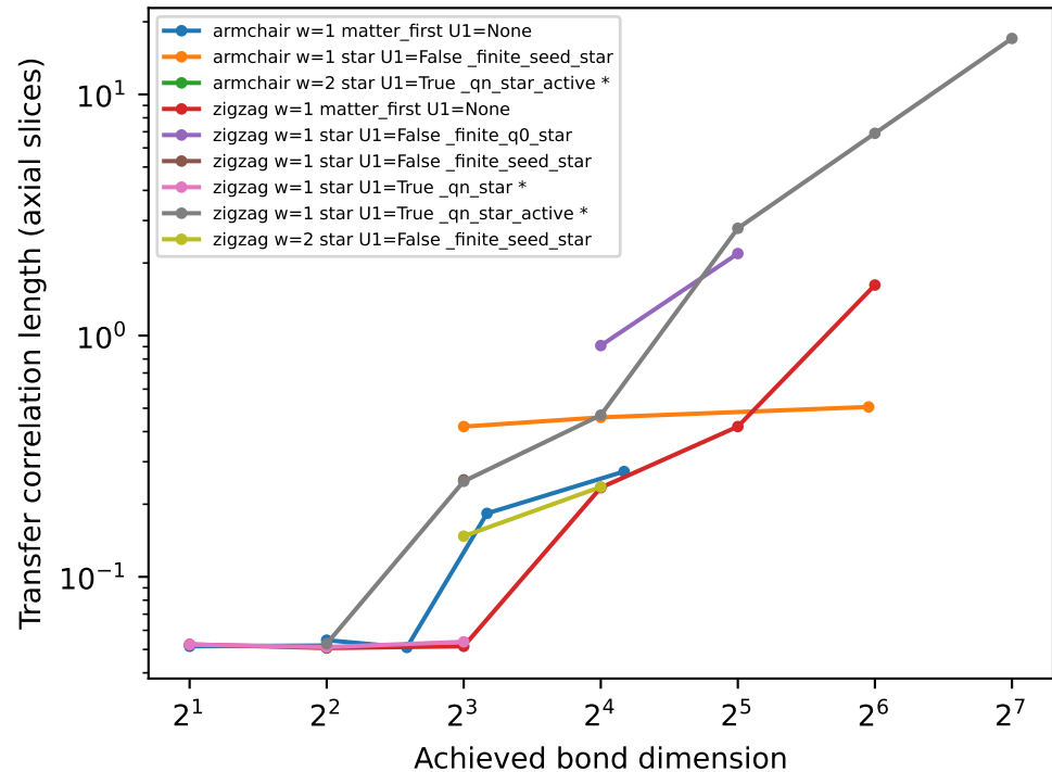
Separate infinite variational branches; * includes energy above a trial bound
