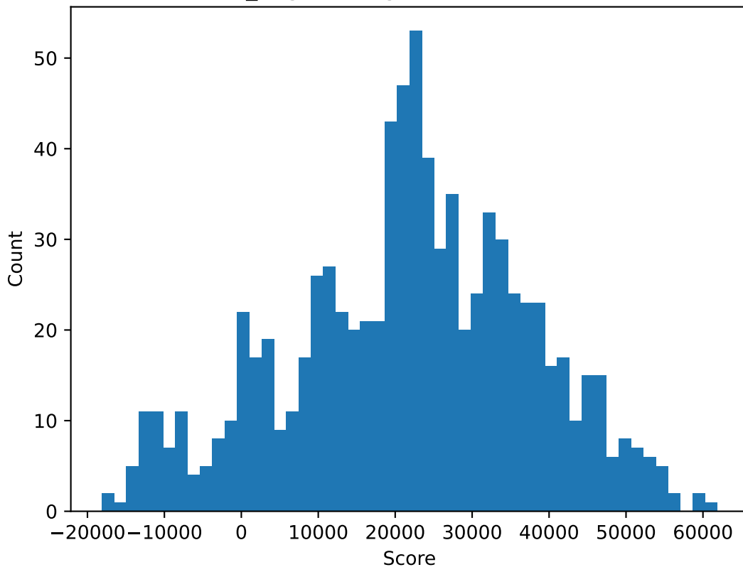
svm_aug Training Scores Distribution
