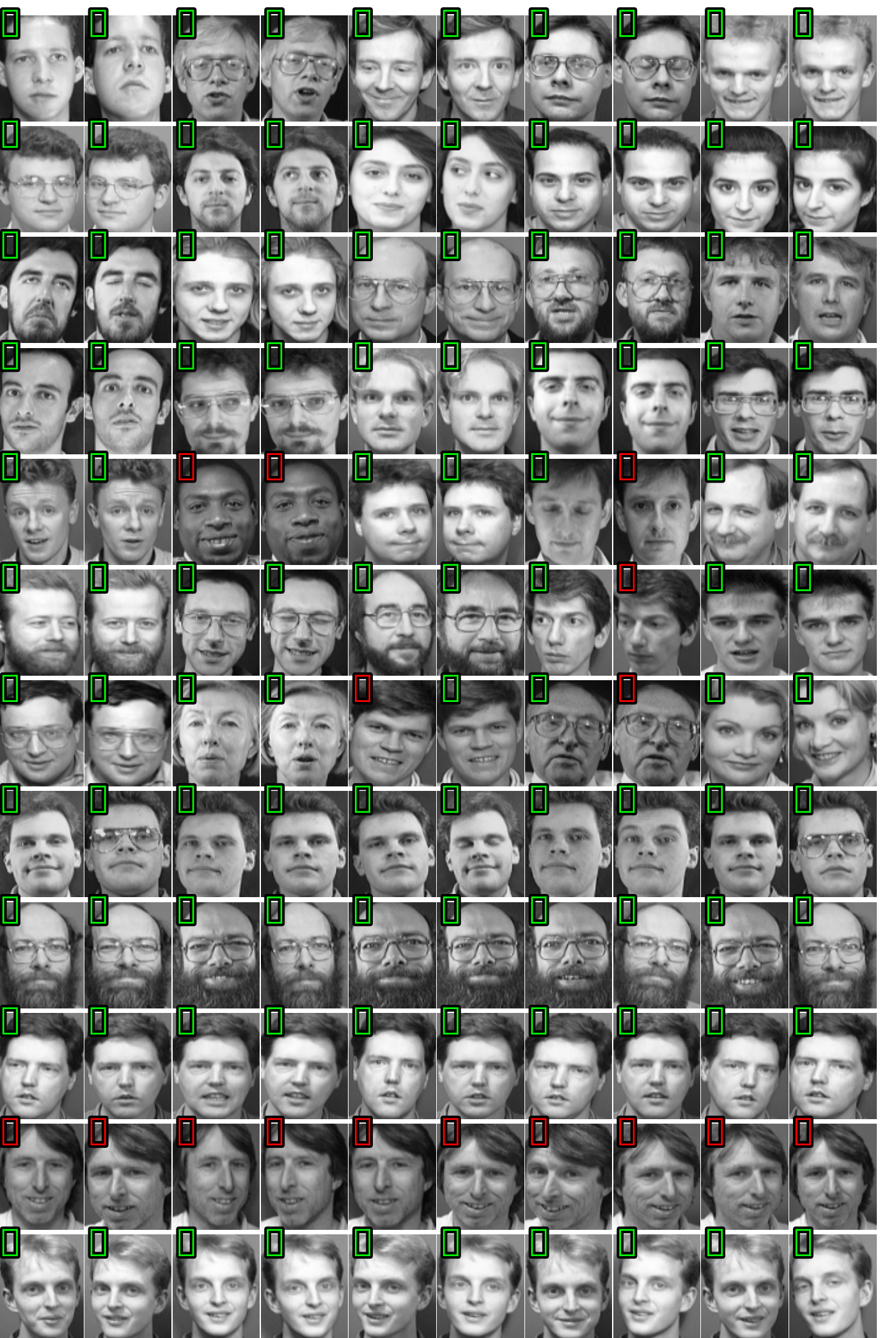
SVM Acc: 86.67%
