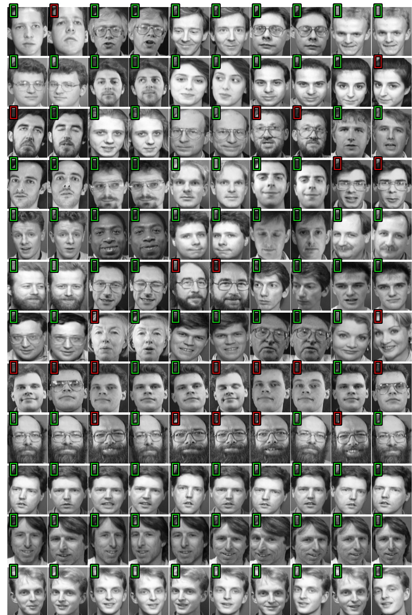
PCA_AUG Acc: 80.83%
