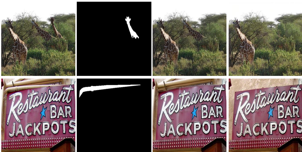
Figure: Comparison of AdaEraser and FLUX.2 [Klein] .The two rows show four columns: the input image, the object mask, the result of AdaEraser, and the result of FLUX.2 [Klein]. For FLUX.2 [Klein], the text instructions are “Remove the rightmost giraffe.” and “Remove the pipe running across the red sign, while keeping the uppermost pipe unchanged.” FLUX.2 [Klein] may remove the wrong target.
