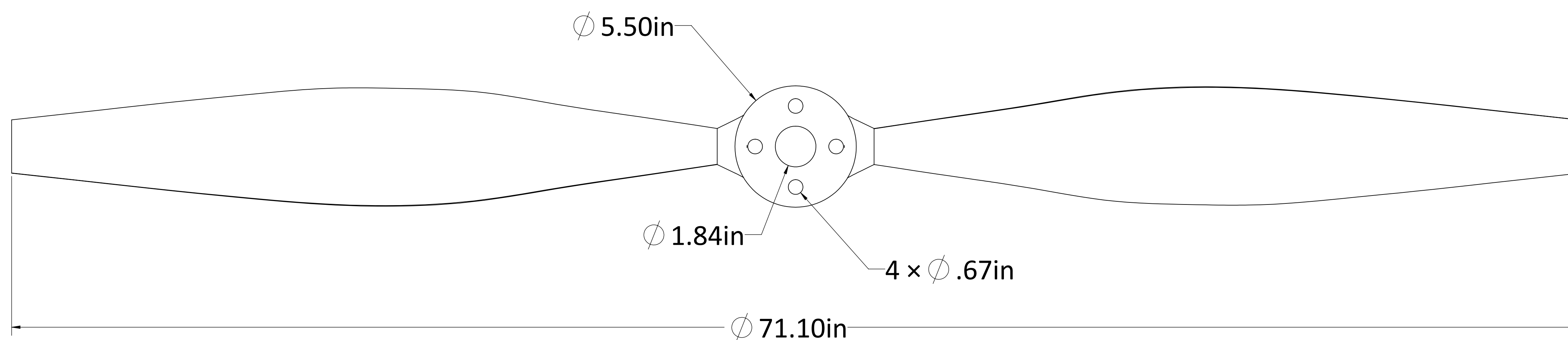
FRONT VIEW
